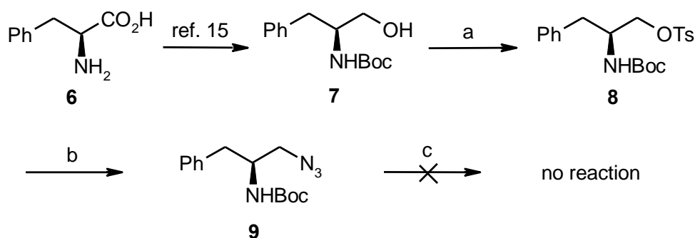
Scheme 1. Reagents and conditions: (a) p -TsCl, Et 3 N, CH_2Cl_2 , 0 °C-rt, 8 h, 88%; (b) NaN_3 , DMF, 70 °C, 6 h, 94%; (c) (i) NaH, BrCH 2 CN, DMF, 0 °C; (ii) K 2 CO 3 , BrCH 2 CN, MeCN, rt; (iii) K 2 CO 3 , BrCH 2 CN, DMF, 80 °C.
