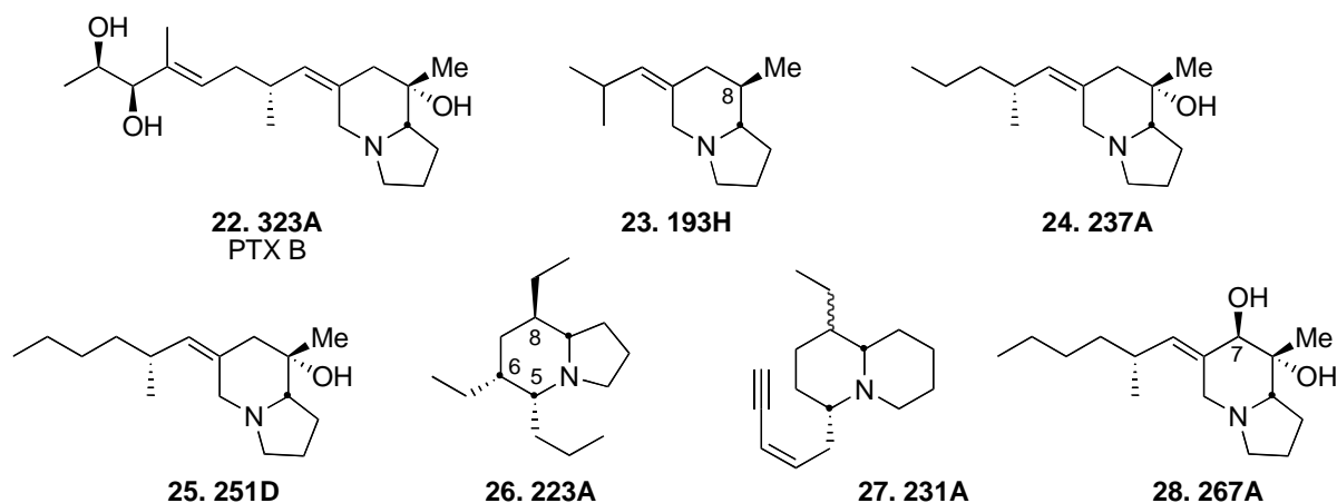
Figure 1. Alkaloid structures.
