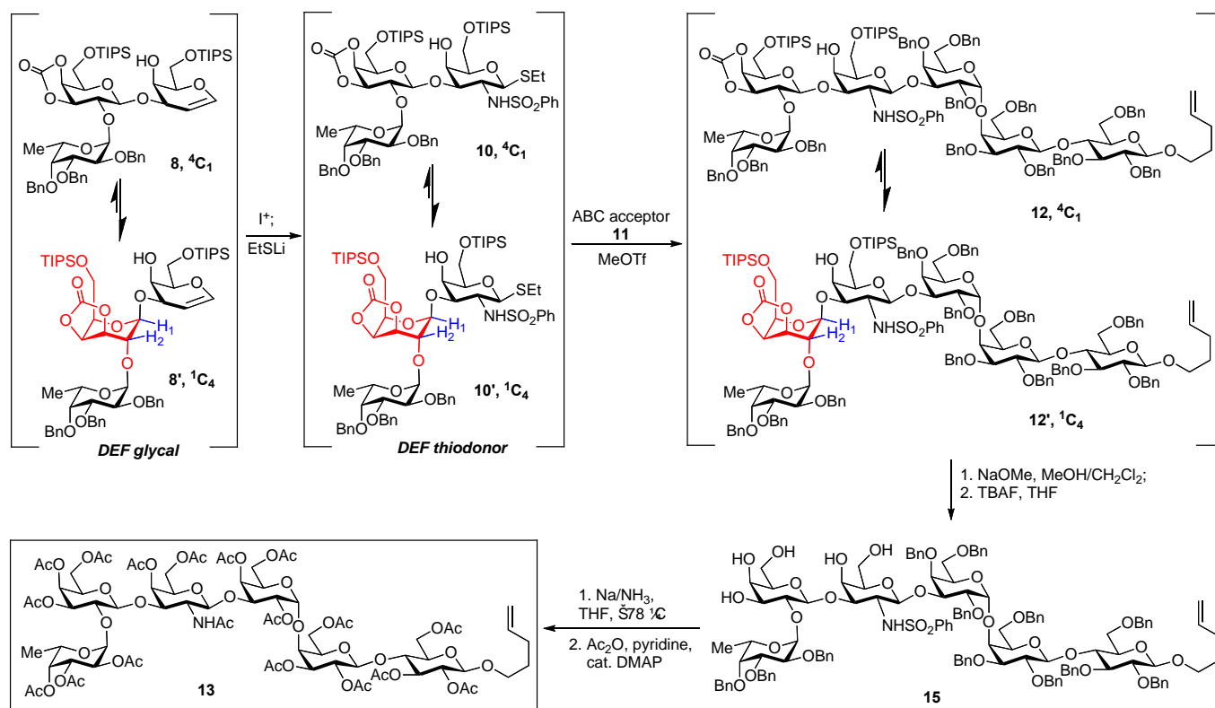
Scheme 2. Conformational reinvestigation.
