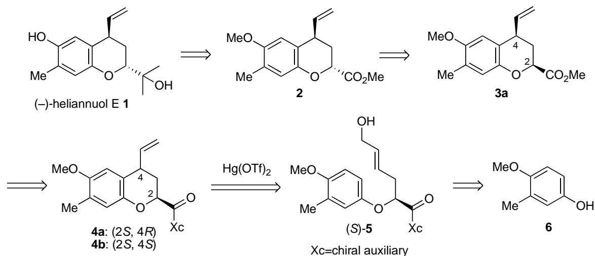
Scheme 1. Retrosynthetic Analysis
