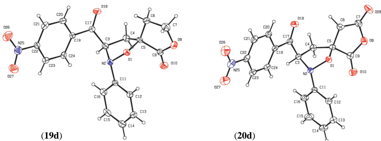
Figure 2. Ortep drawing of molecule ( 19d ) and ( 20d ), drawn by program PLATON . 32 Displacement ellipsoids are shown at the 20% probability level. Comparison of torsion angle values shows that the isoxazolidinic ring adopts the same half-chair conformation, in which atoms N2 and C3 are respectively deviated, by -0.347(3) and 0.293(3) Å from the mean plane of the other three atoms in ( 19d ), by -0.288(2) and 0.329(2) Å, in ( 20d ).
