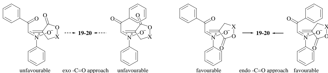
Scheme 6. Endo - C=O and exo - C=O transition states for the reaction of C -aroyle- N -phenylnitrones ( 7a-d ) with 3-methylenedihydro-(3 H )-furan-2-one ( 1 ) and itaconic anhydride ( 2 ).
