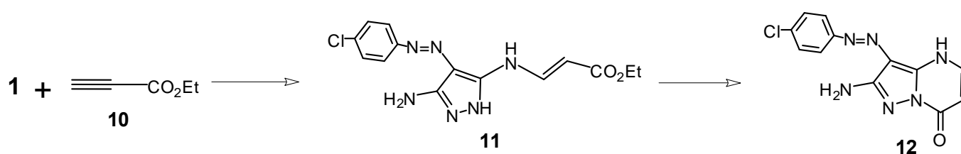
Scheme 3
