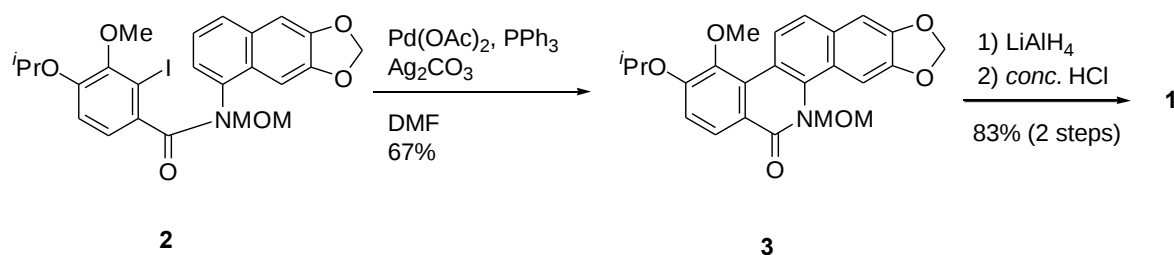
Scheme 1 Synthesis of 1
