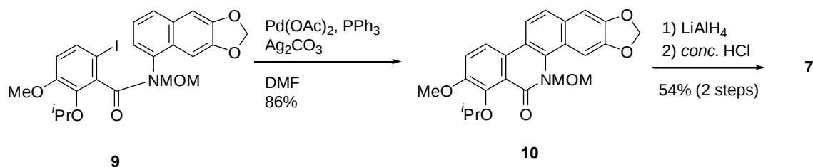
Scheme 3 Synthesis of 7
