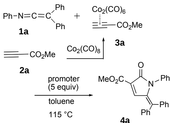
Scheme 1. Efficiency of promoters in a model P-K reaction between 1a and 3a .
