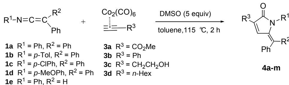
Scheme 2. Scope of the ketenimine Pauson–Khand reaction to give \gamma -lactams 4 .
