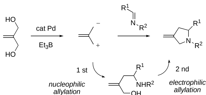
Scheme 2. Amphiphilic Allylation of Aldimine
