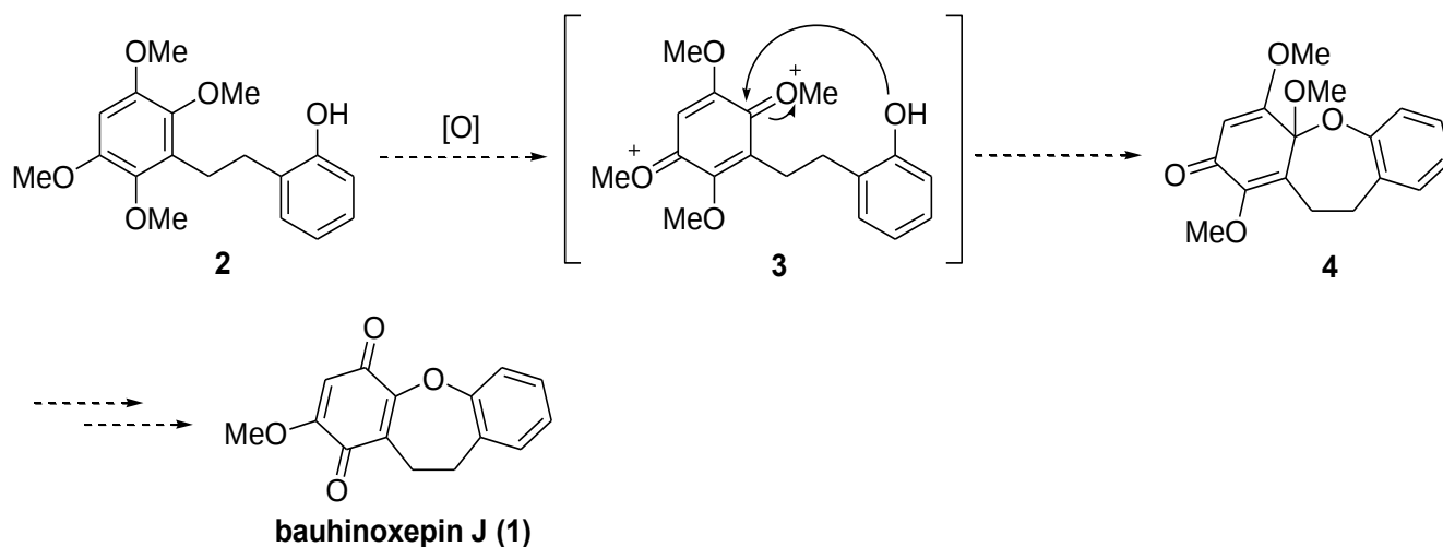
Scheme 1. Approach to baughinoxepin J ( 1 )
