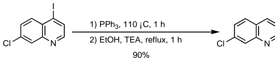
Scheme 4 The one-pot conversion of 7-chloro-4-iodoquinoline into 7-chloroquinoline
