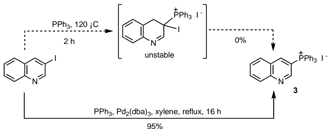
Scheme 3 Preparation of 3-quinolinyltriphenylphosphonium iodide ( 3 ) by palladium coupling reaction
