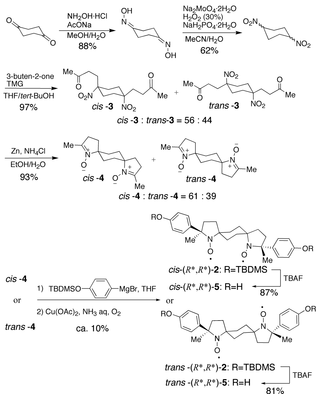
Scheme 1. Preparation of racemic cis-(R^*,R^*)-2 and trans-(R^*,R^*)-2
