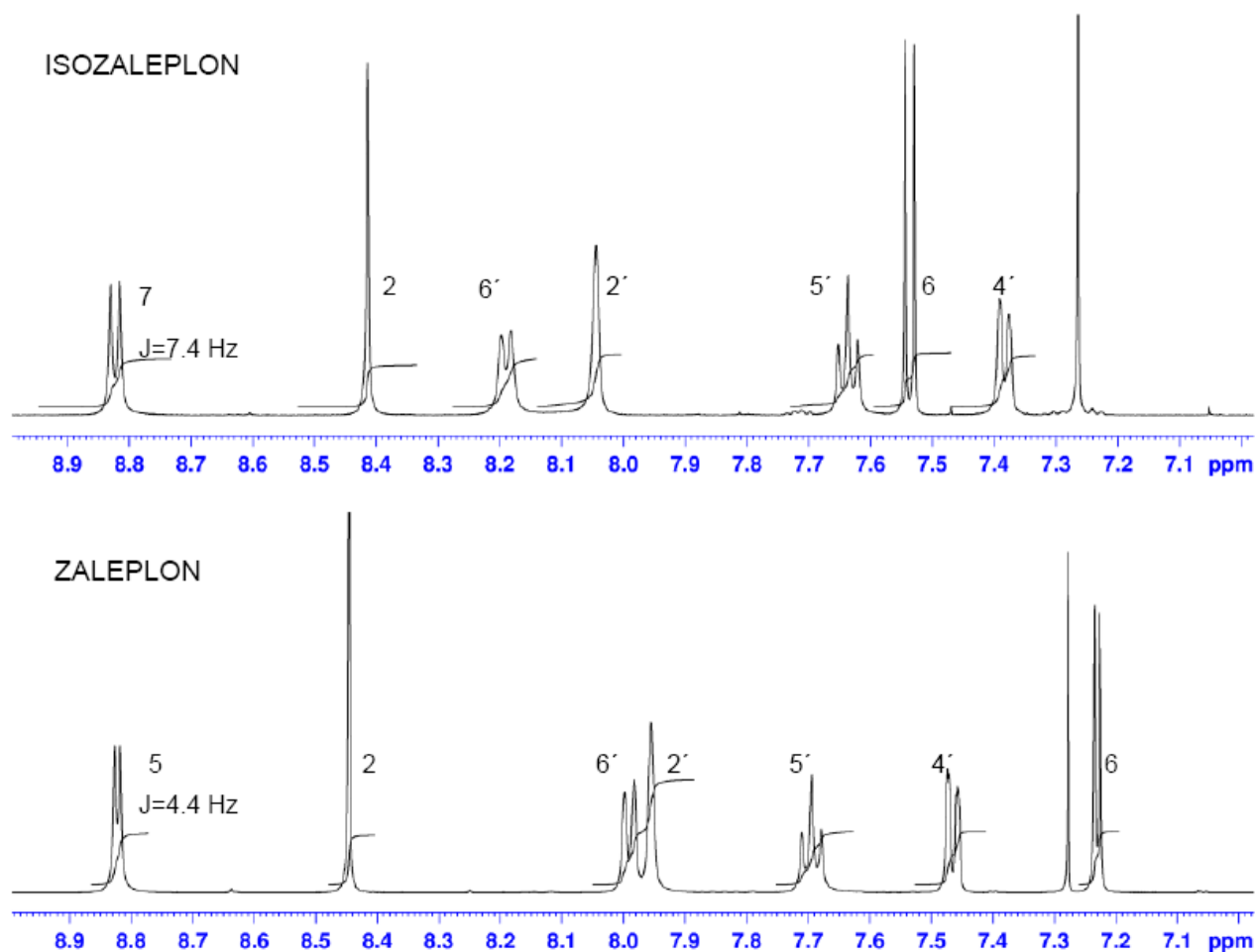
Figure 1 Comparison of aromatic regions of proton spectra for isozaleplon ( 4 ) and zaleplon ( 1 ).
