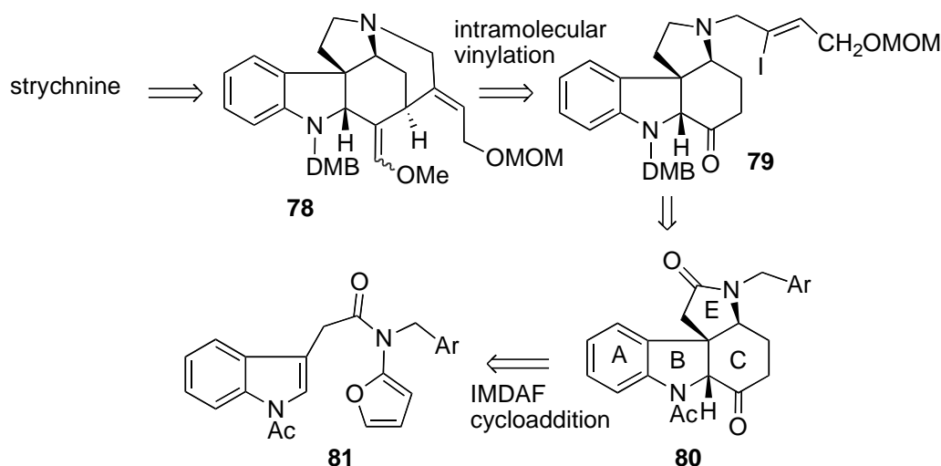
Scheme 16. Retrosynthetic Analysis of ( \pm )-Strychnine
