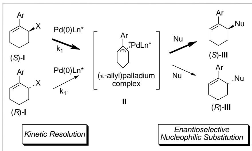
Scheme 26. Reaction Pathways
