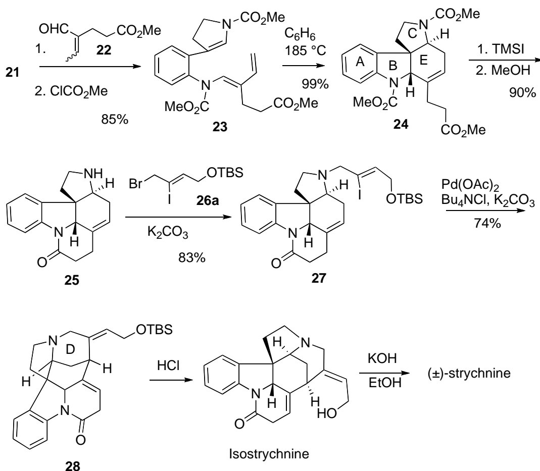
Scheme 4. Rawal's Total Synthesis of (±)-Strychnine
