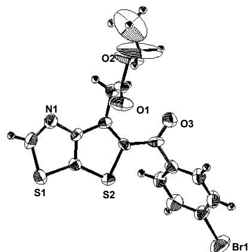
Figure 1. ORTEP drawing of 3I
