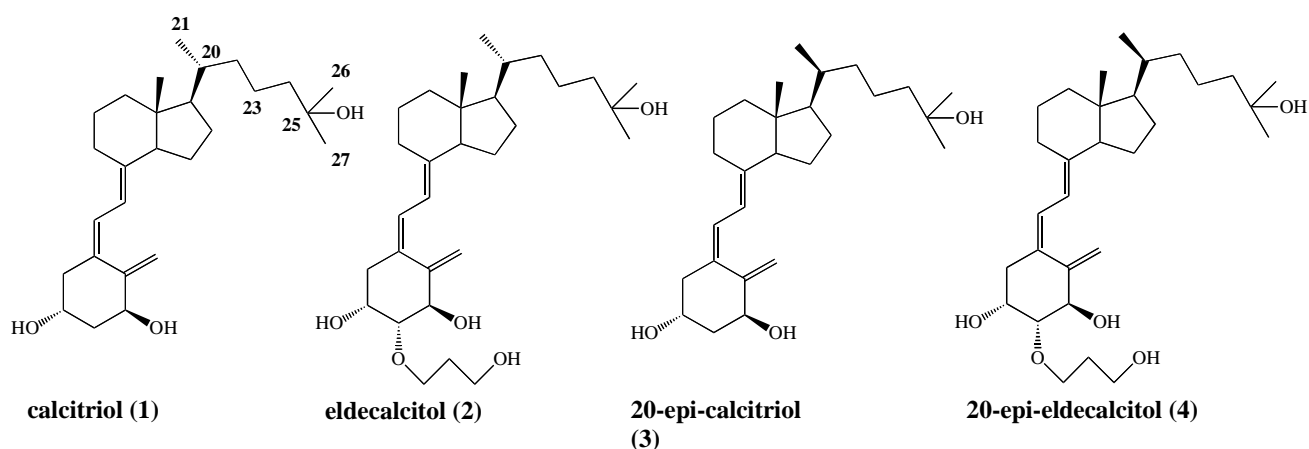
Figure 1. Structures of calcitriol, eldecalcitol, 20- epi -calcitriol, and 20- epi -eldecalcitol
