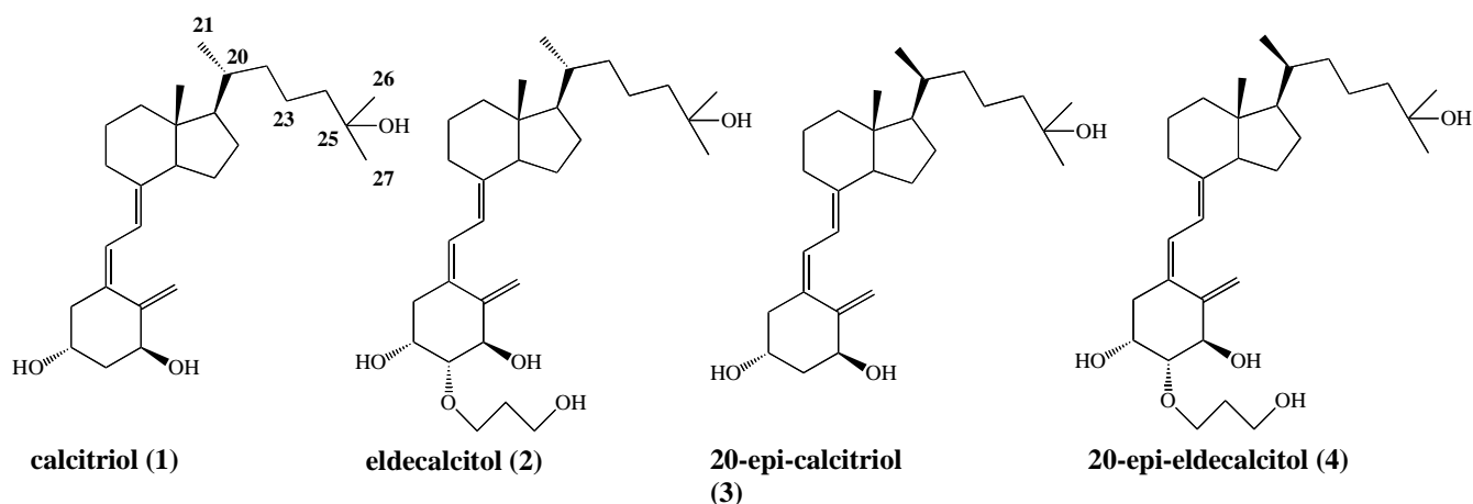
Scheme 1. Retrosynthesis of 20-epi-eldecalcitol (4).
