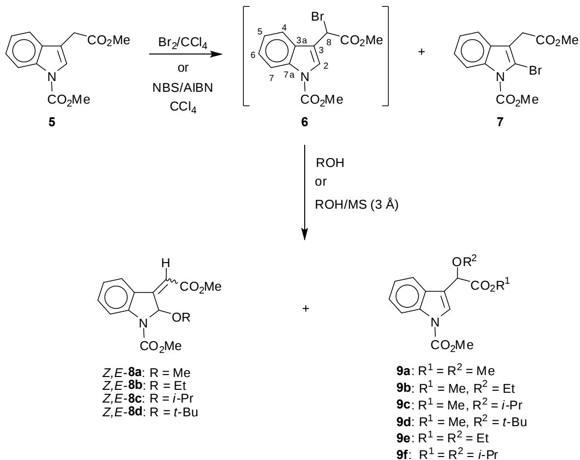
Scheme 2. Synthesis of (Z)- and (E)-2-alkoxyindolenines 8 , and 3-indolyl(alkoxy)acetates 9 .
