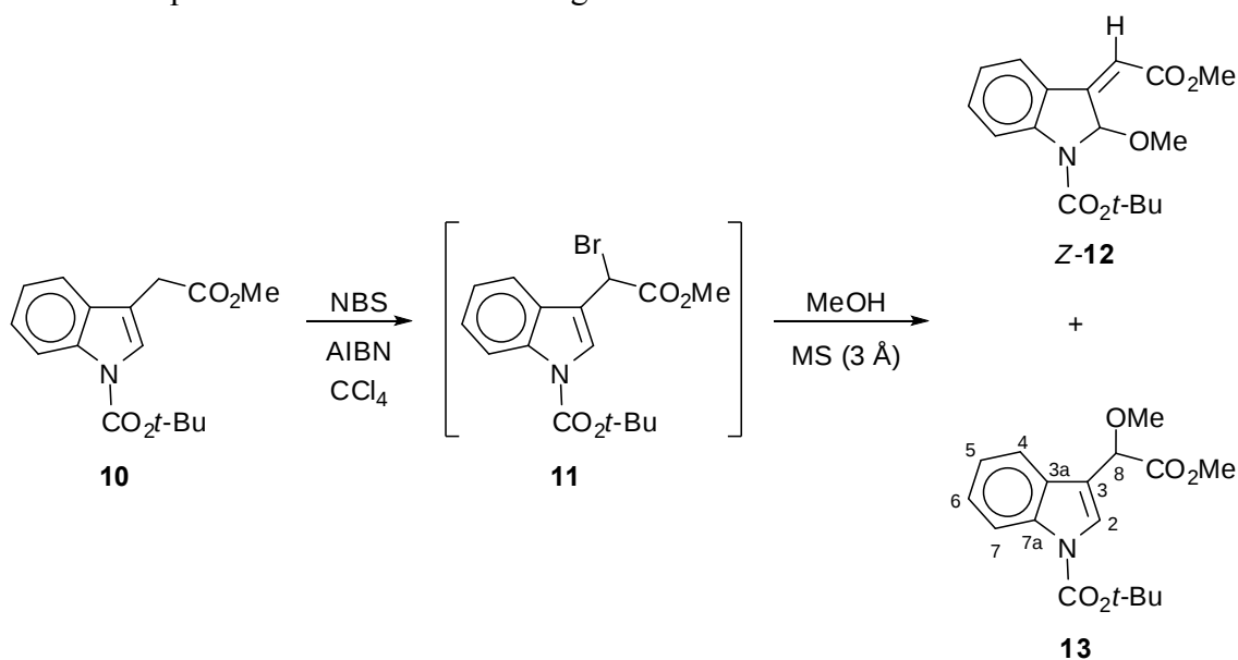
Scheme 3
