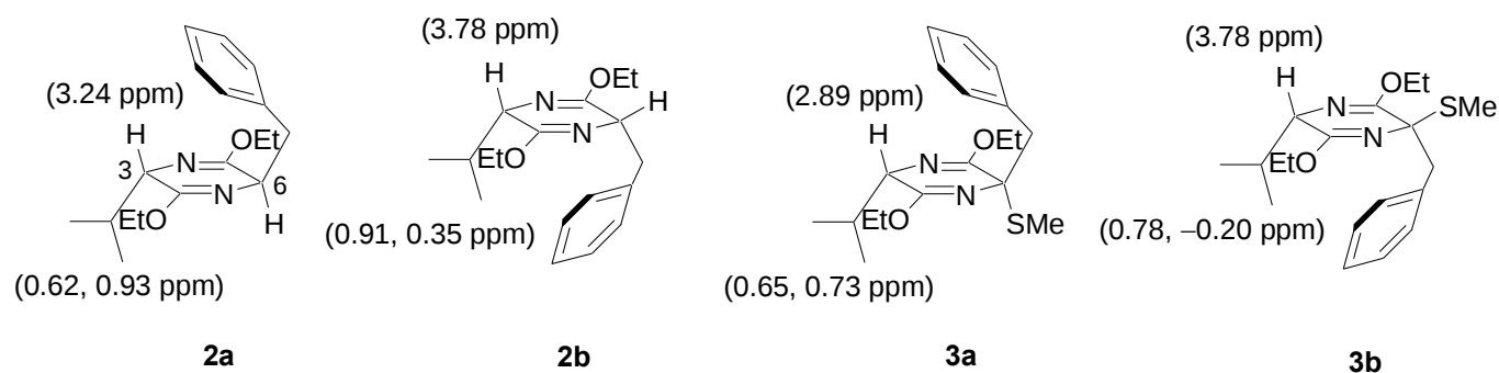
Figure 2. Conformations and ^1\text{H} -NMR chemical shifts of 2 and 3
