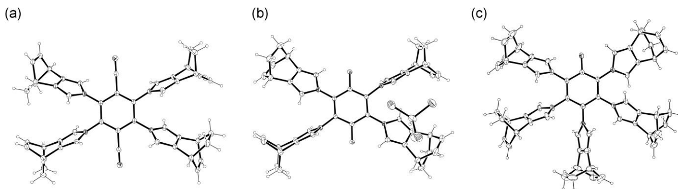
Figure 1. Ortep drawing of 3a (a), 3b ·2CHCl 3 (b), and 4 (c). Disordered atoms are omitted for clarity
