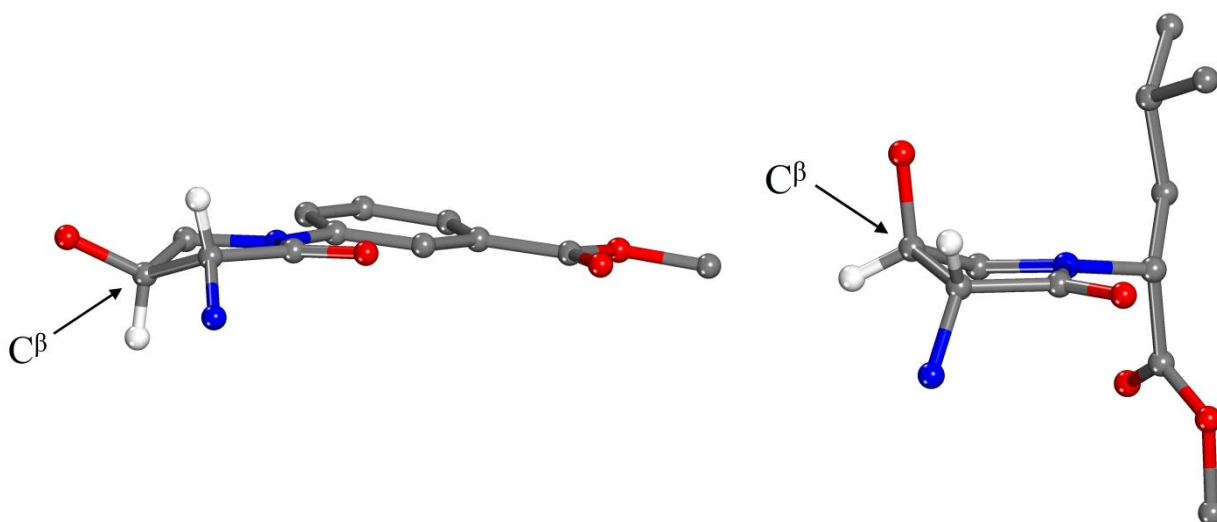
Figure 5. Endo and exo puckering of the C β atom in 4a (left) 4b (right) respectively. All hydrogens except those at C α and C β , the Fmoc groups, and the benzene solvent in 4a have been omitted for clarity
