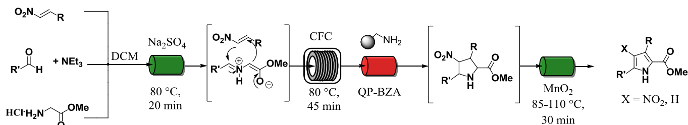
Scheme 3. Multistep flow set-up towards nitropyrrole products
