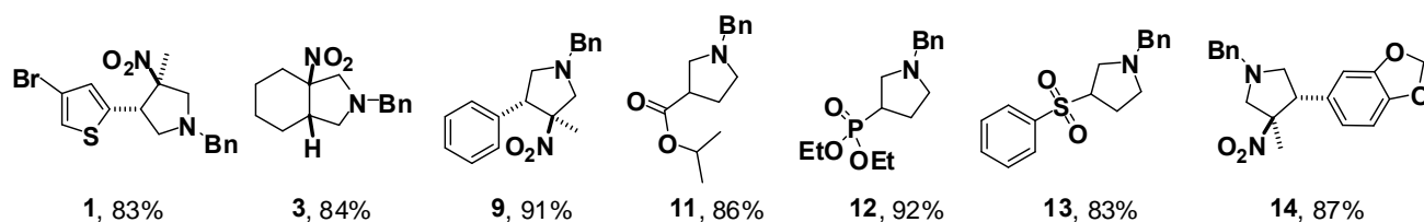
Figure 2. 3-Nitropyrrolidines prepared using a fluoride-monolith
