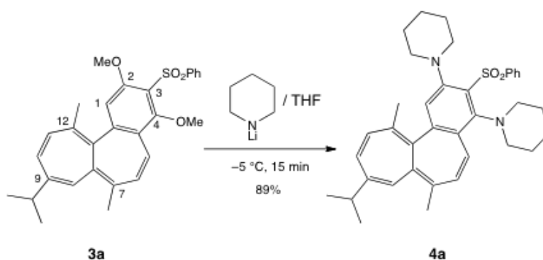
Scheme 2. Formation of 4a by nucleophilic substitution
