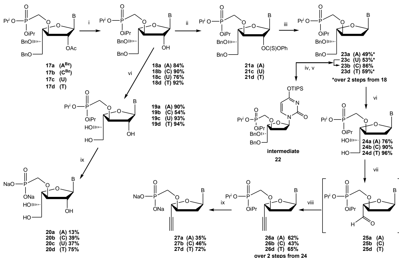
Scheme 2. i) \text{MeOH}/\text{NH}_3 overnight, RT; ii) \text{PhOC(S)Cl} , DMAP, \text{MeCN} , 0\text{ }^\circ\text{C} ; iii) AIBN, \text{Bu}_3\text{SnH} , toluene, reflux; iv) DMAP, \text{E}_3\text{N} , TIPS \text{Cl} , \text{CH}_2\text{Cl}_2 , RT overnight; 88% yield; v) \text{NH}_3 solution in dioxane, RT, 5 h; vi) cyclohexene, \text{Pd}(\text{OH})_2 , \text{MeOH} , 80\text{ }^\circ\text{C} ; vii) \text{NaIO}_4 , aq \text{MeOH} RT; viii) \text{MeCOC(N}_2\text{)P(O)(OMe)}_2 ( 28 ), \text{K}_2\text{CO}_3 , \text{MeOH} , RT; ix) TMSI, 2,6-lutidine, \text{MeCN} ;
