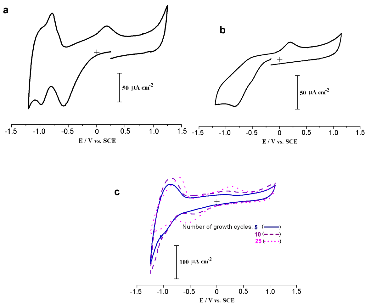
Figure 4. Redox behaviour of the modified electrodes in 0.1 M LiClO 4 /MeCN; v = 50 \text{ mV/s} . a: Pt electrode coated with P(B 12 -Ty) (4 potential cycles with 60 s delay at -1.2 V); b: GC coated with P(B 12 -Ty) (10 potential cycles with 60 s delay at -1.2 V); c: Pt-(P-Ty)/P(B 12 -Ty) electrode.
