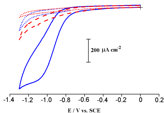
Figure 7. Voltammetric responses of bare (red) and modified GC-P(B 12 -Ty) (blue) electrodes in phosphate buffer solution with 10 mM KNO 2 (full/broken line) and without 10 mM KNO 2 (dotted line), \nu = 50 mV/s.
