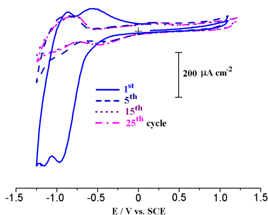
Figure 3. Cyclic voltammograms of B 12 -Ty (2) (1 mM) at a Pt electrode, Pt-(P-Ty)/P(B 12 -Ty), with a preformed polytyramine film in a 0.1 M LiClO 4 /CH 3 CN solution; \nu = 50 mV/s.
