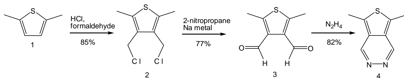
Scheme 1. Synthesis of 5,7-dimethylthieno[3,4- d ]pyridazine ( 4 )
