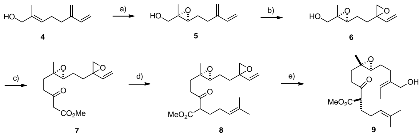
Scheme 3. Reagents and conditions: a) \text{Ti}(\text{O}i\text{Pr})_4 , L-(+)-DET, TBHP, MS4A, \text{CH}_2\text{Cl}_2 , -35^\circ\text{C} , 99% (92% ee); b) MCPBA, \text{CH}_2\text{Cl}_2 , 0^\circ\text{C} , 91%; c) \text{Tf}_2\text{O} , \text{Et}_3\text{N} , THF, -78^\circ\text{C} , then 5 eq. the dianion of methyl acetoacetate generated with NaH and n\text{BuLi} , THF, 0^\circ\text{C} , 94%; d) NaH, 15-crown-5, DMSO, then 5-iodo-2-methylpent-2-ene, 77%; e) 10 mol% \text{Pd}(\text{PPh}_3)_4 , DMSO, 90^\circ\text{C} , 60%.
