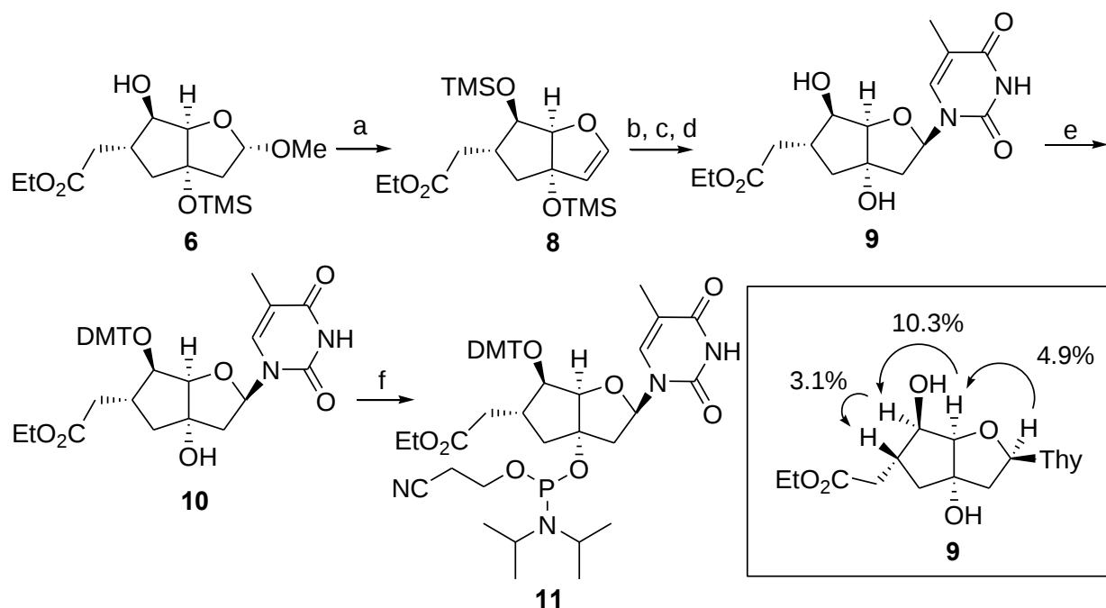
Scheme 2. Synthesis of building block 11 and ^1\text{H} -NMR difference NOE effects observed for nucleoside 9 . Conditions: a) 2,6-lutidine, TMS-OTf, \text{CH}_2\text{Cl}_2 , 1h, rt, quant.; b) thymine, BSA, NIS, rt, 3h; c) AIBN, \text{Bu}_3\text{SnH} , toluene, 95^\circ\text{C} , 2h; d) HF-pyridine, pyridine, rt, 4h, 13% from 6 ; e) DMT-OTf, pyridine, rt, 13h, 72%; f) (i\text{Pr}_2\text{N})\text{P}(\text{Cl})\text{OCH}_2\text{CH}_2\text{CN} , \text{CH}_3\text{CN} , (i\text{Pr})_2\text{NEt} , rt, 1h, 60%.
