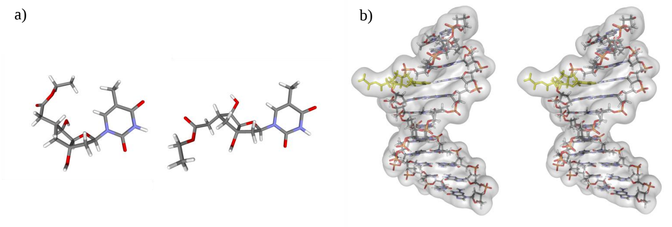
Figure 2. a) The two low energy conformers found for bc^{\alpha\text{-alk}}\text{-T} nucleoside; b) stereo view of a DNA duplex model containing one bc^{\alpha\text{-alk}}\text{-T} residue (yellow) in one DNA strand.
