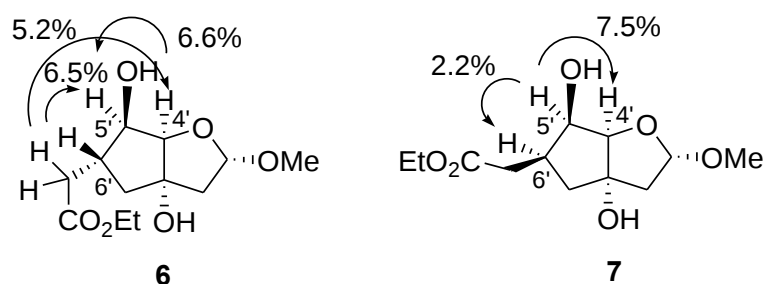
Figure 3. intensity of observed (mutual) ^1\text{H} -NMR difference NOE effects of the relevant protons used for assigning the cis - and trans -relationship of substituents in the carbocyclic ring in 6 and 7 .
