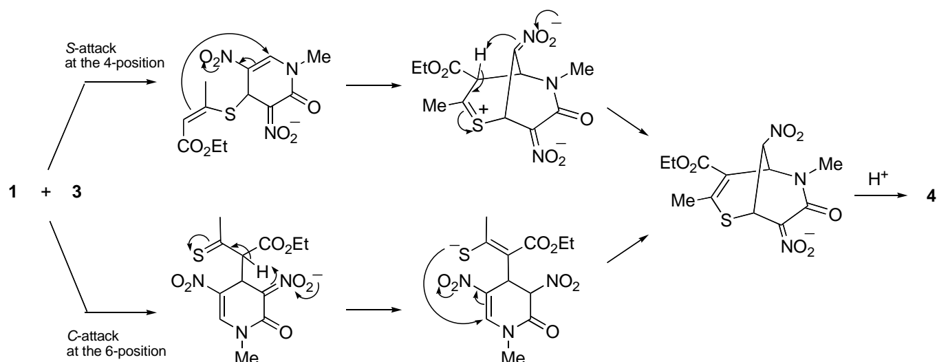
Scheme 2. Plausible mechanism
