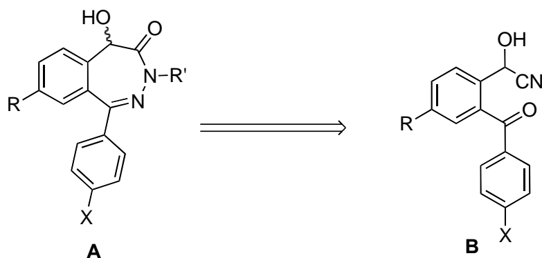
Scheme 1. Retrosynthetic analysis A ⇒ B
