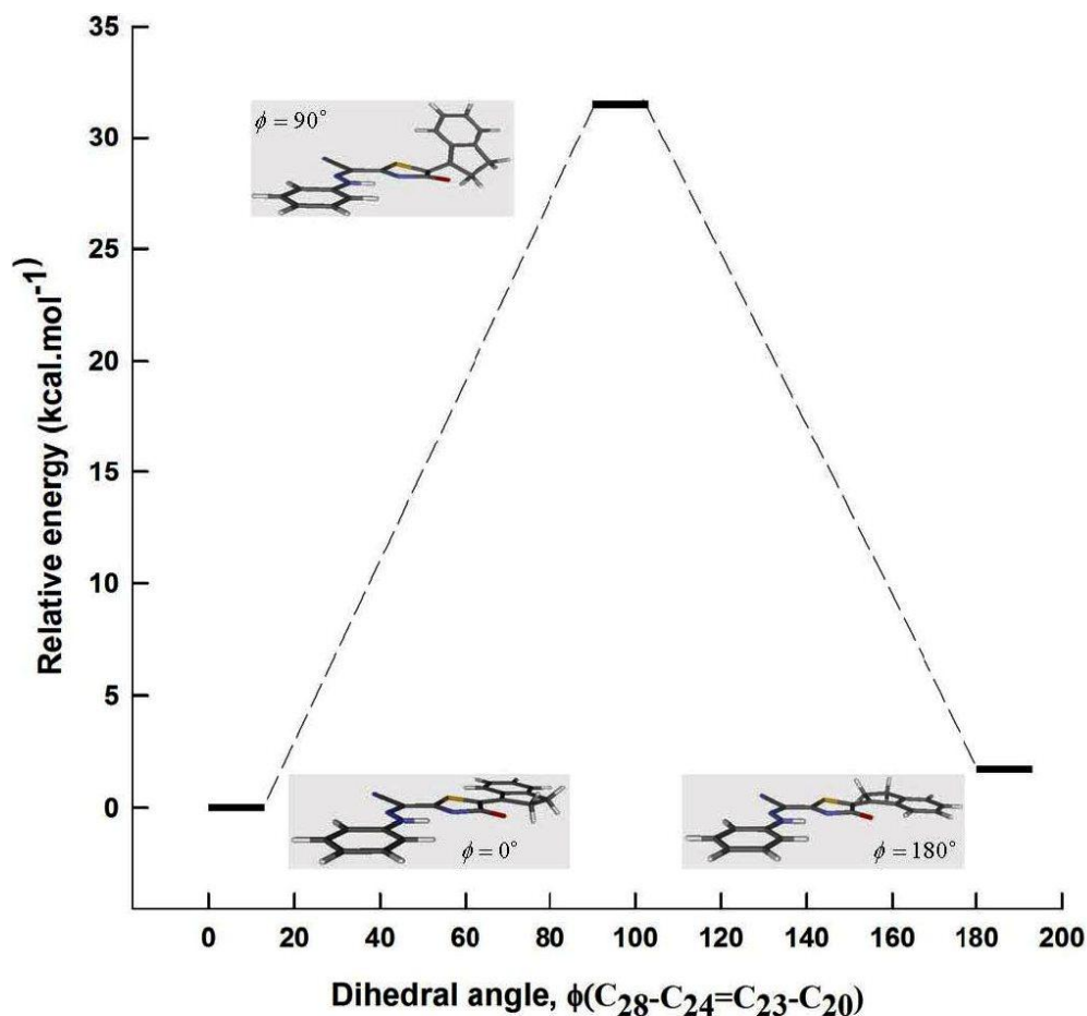
Figure 3. The energy barrier for rotation of the bicyclic 1H-indan-1-ylidene moiety in compound 6e around the C 23 =C 24 double bond.
