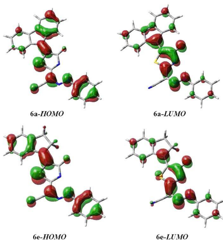
Figure 4: The HOMO and LUMO of compounds 6a and 6e .
