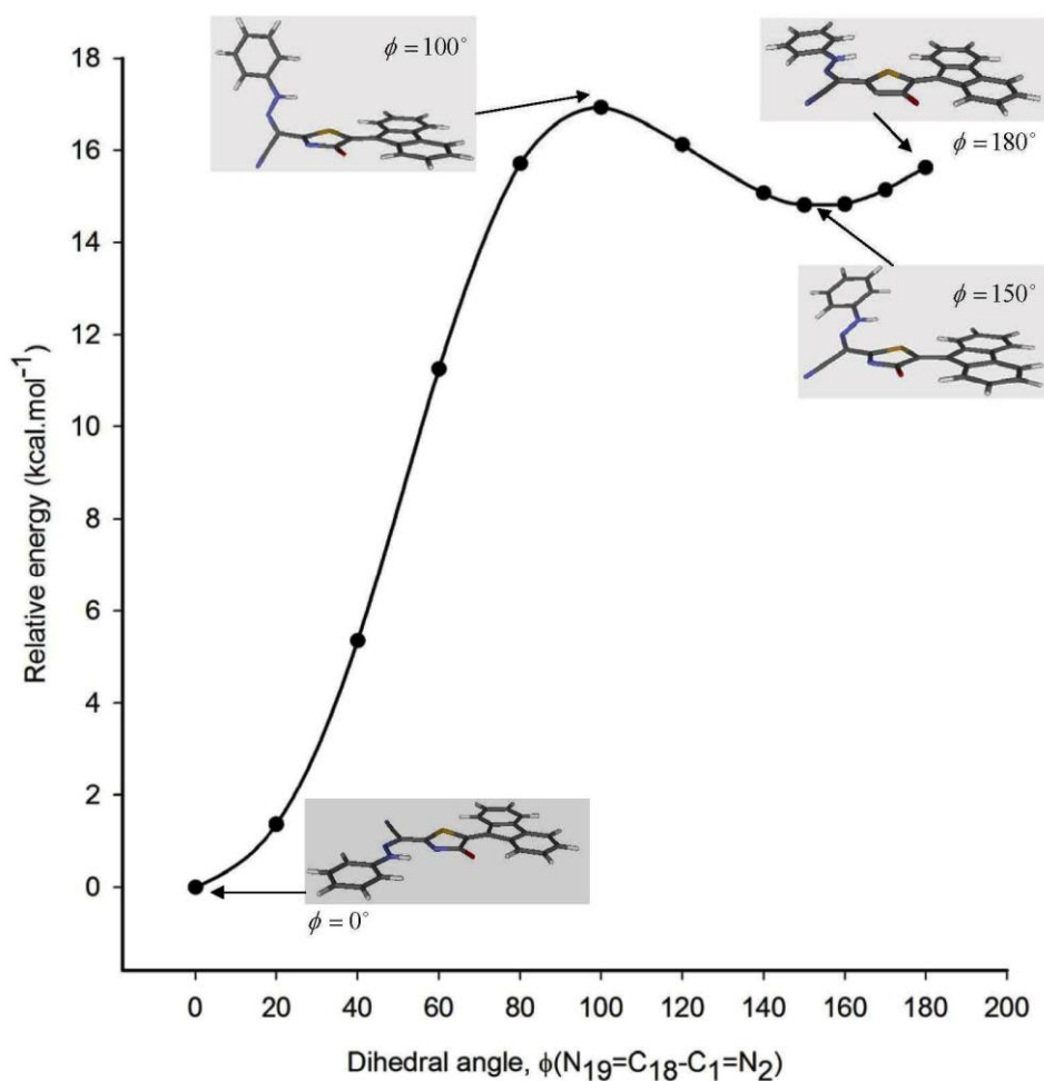
Figure 2. Energy profile for rotation around the C_{18}-C_1 single bond of compound 6a
