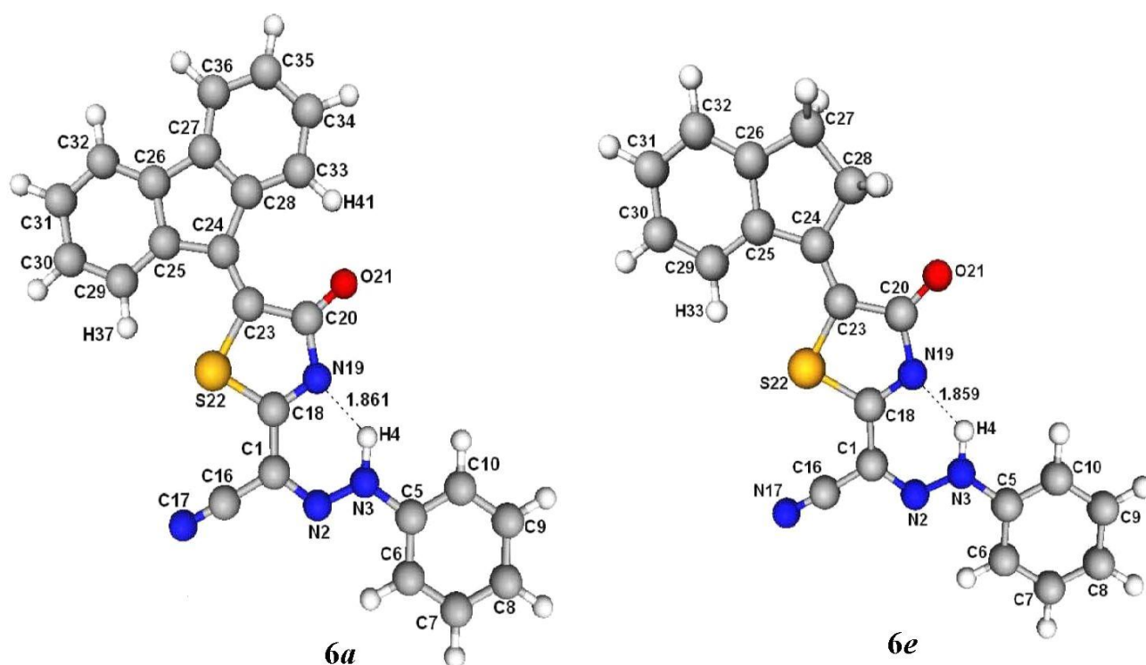
Figure 1. B3LYP/6-31G(d) optimized structures of compounds 6a and 6e . Numbering systems are included.
