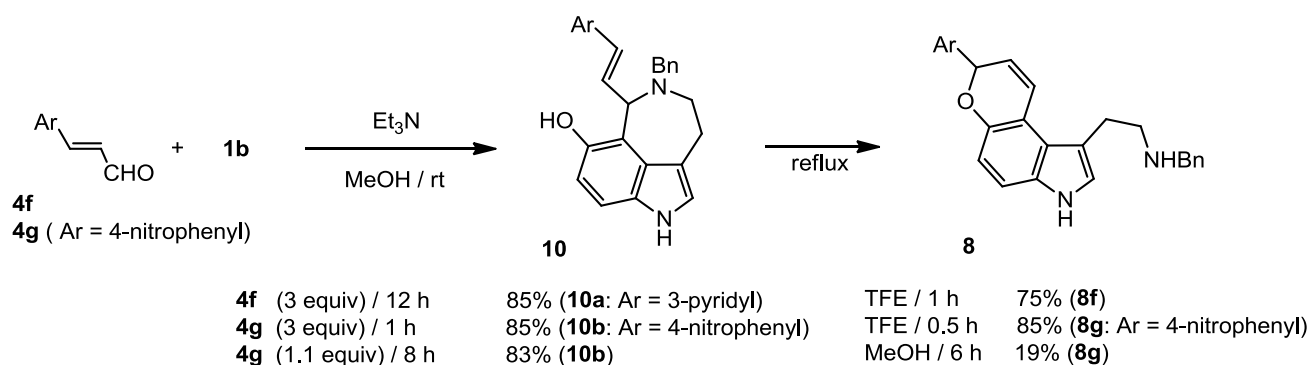
Scheme 2
