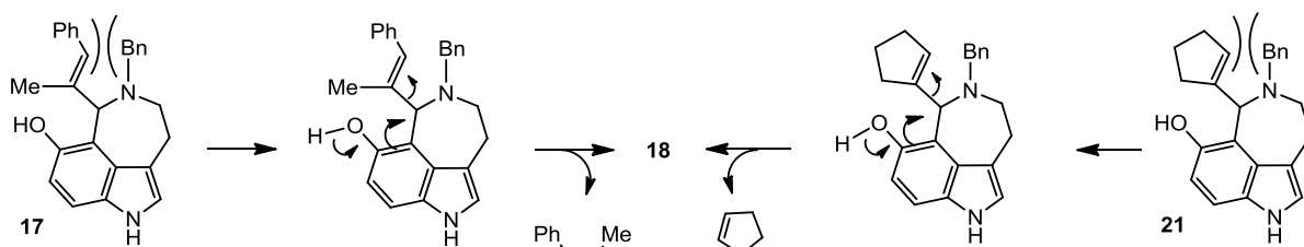
Scheme 5
