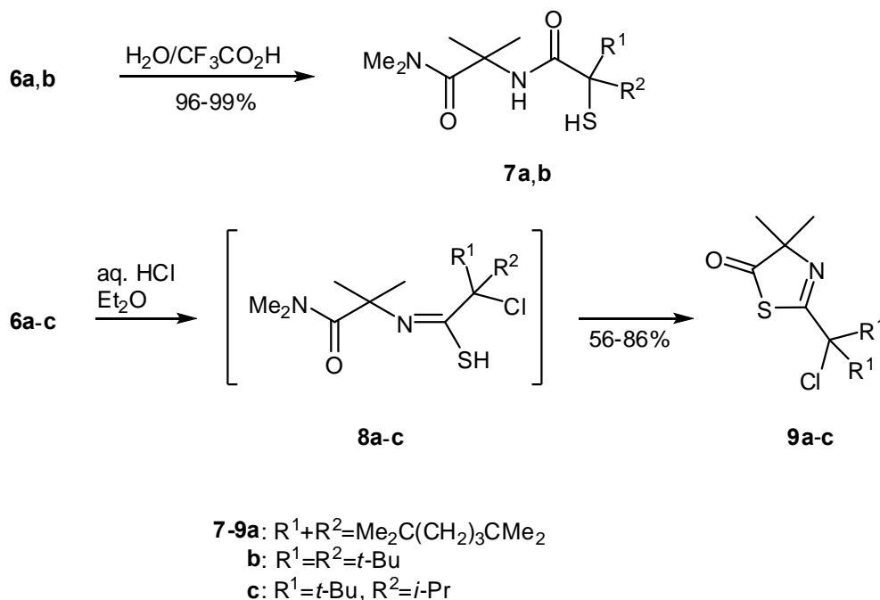
Scheme 2. Attack of simple nucleophiles on thiiranimines 6
