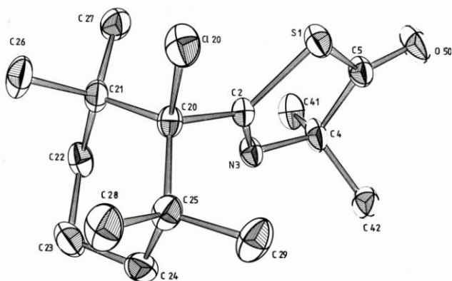
Figure 1. Perspective ORTEP presentation of the molecular structure of thiazolinone 9a (hydrogen atoms not shown)
