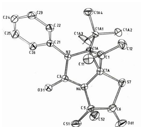
Figure 7. Perspective ORTEP presentation of the molecular structure of tricyclic 21 (hydrogen atoms not shown)
