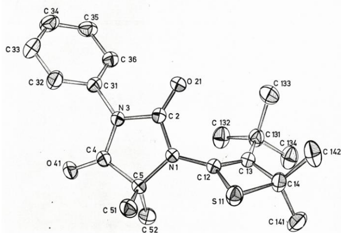
Figure 6. Perspective ORTEP presentation of the molecular structure of thiete 19a (hydrogen atoms not shown)
