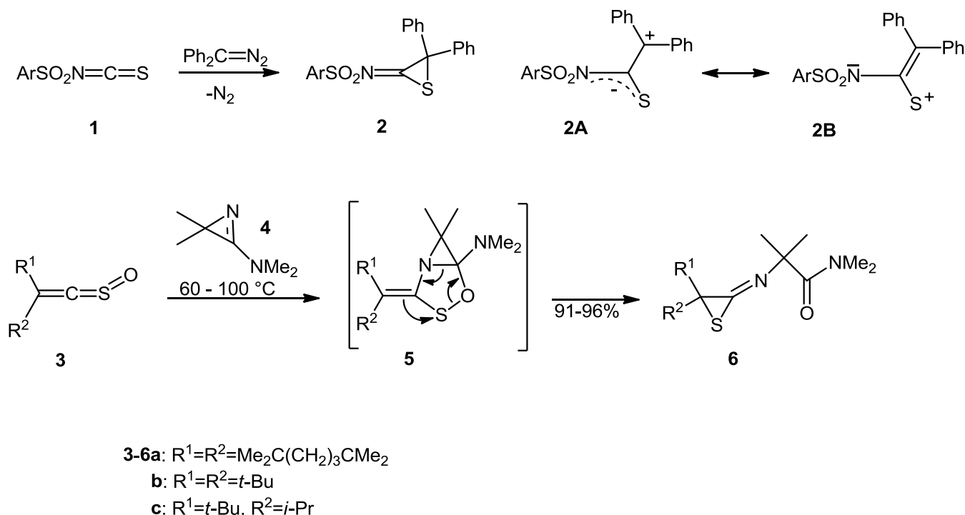
Scheme 1. Syntheses of thiiranimines 2 , 6
