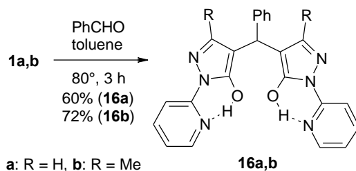
Scheme 5. Reaction of 1a,b with benzaldehyde
