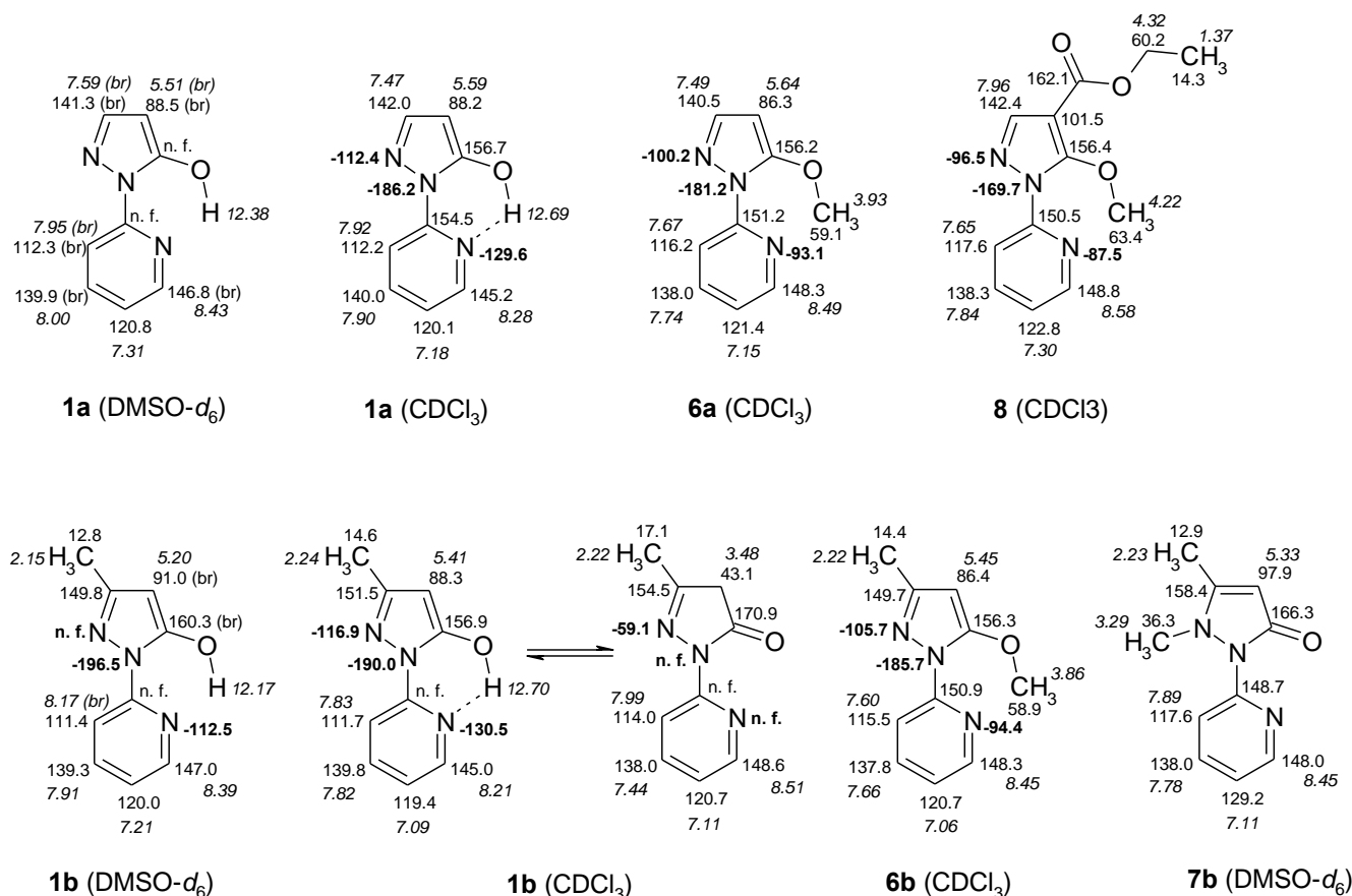
Figure 2. ^1\text{H} (italics), ^{13}\text{C} and ^{15}\text{N} -NMR (bold) chemical shifts in 1a,b and fixed derivatives 6a,b , 7b and 8 (n. f. = not found, br = broad signal)
