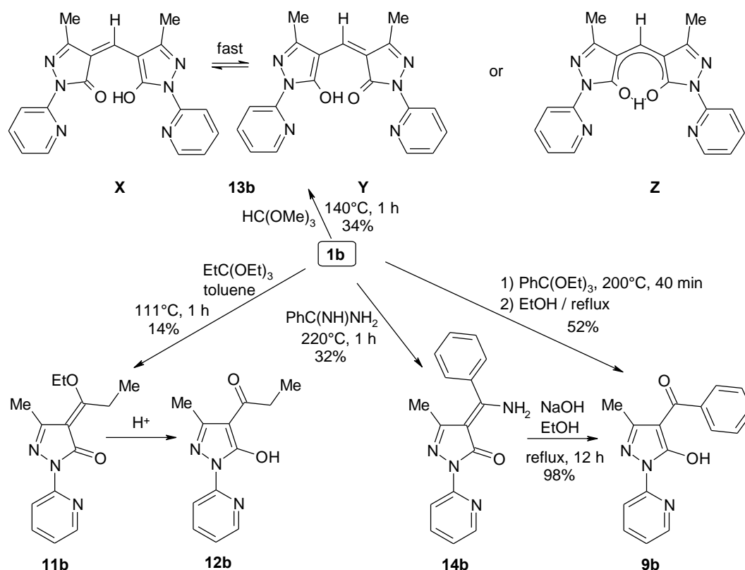
Scheme 3. Reaction of 1a,b with orthoesters and benzamidine
