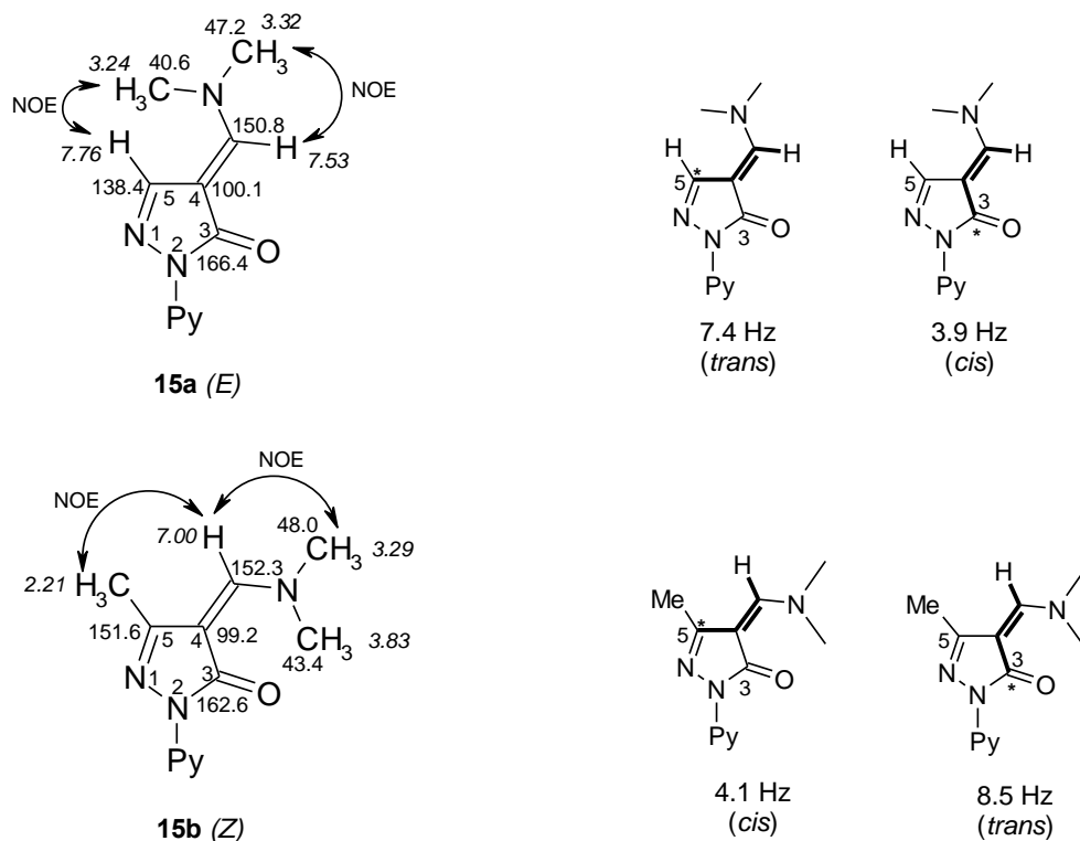
Figure 4. Determination of the stereochemistry of compounds 15 via NOEs (arrows), ^1\text{H} (italics) and ^{13}\text{C} -NMR chemical shifts as well as ^{13}\text{C} , ^1\text{H} coupling constants
