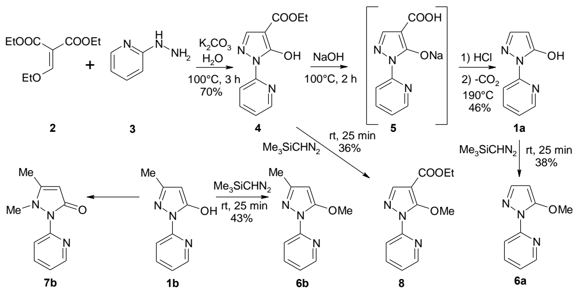
Scheme 1. Synthesis of pyrazolone 1a and 'fixed' forms 6a , 6b , 7b and 8
