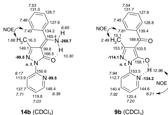
Figure 3. ^1\text{H} (italics), ^{13}\text{C} and ^{15}\text{N} -NMR (bold) chemical shifts in 14b and 9b (n. f. = not found)
