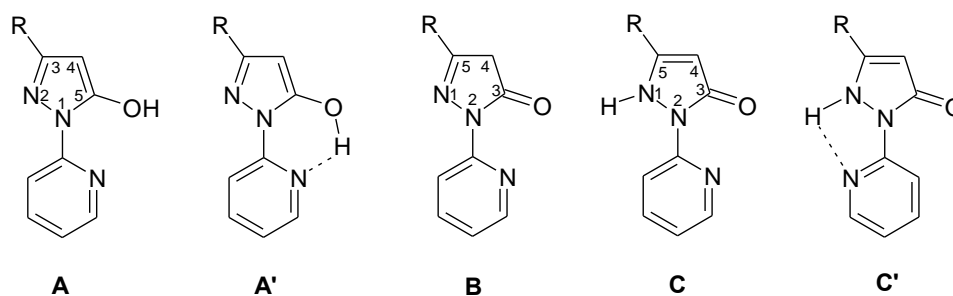
Figure 1. Possible tautomeric forms of title compounds 1
