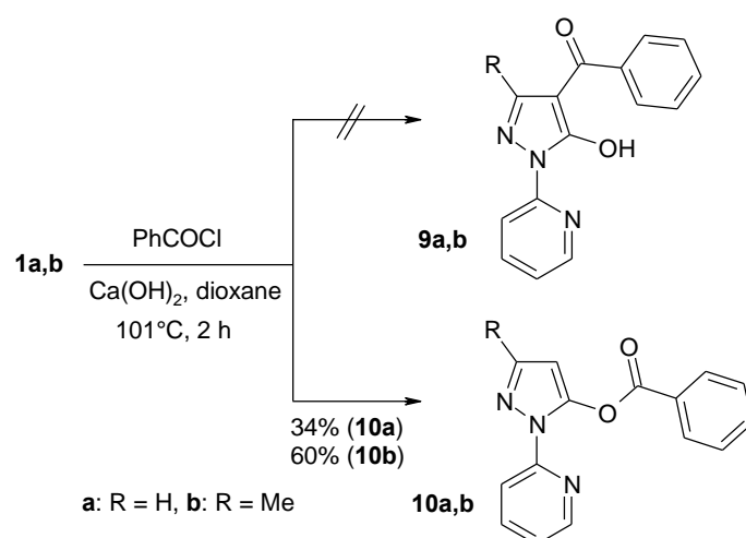
Scheme 2. Reaction of 1a,b with benzoyl chloride / \text{Ca(OH)}_2
