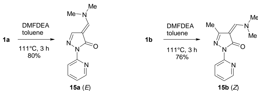
Scheme 4. Reaction of 1a,b with DMFDEA
