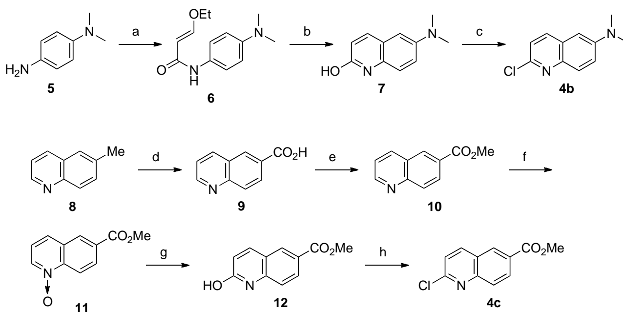
Scheme 2. Syntheses of 6-substituted-2-chloroquinoline derivatives 4b and 4c . Reagents and Conditions: a) 3-ethoxypropenylchloride, Et 3 N, toluene, reflux, 2 h, 57%; b) conc. H 2 SO 4 , 50 °C, 24 h, 45%; c) POCl 3 , reflux, 3 h, 58%; d) CrO 3 , conc. H 2 SO 4 , H 2 O, reflux, 24 h, 40% (based on recovered 8 ); e) p -TsOH, MeOH, reflux, 24 h, 99%; f) m CPBA, CHCl 3 , rt, 18 h, 94%; g) Ac 2 O, 100 °C, then H 2 O, rt, 72 h, 74%; h) POCl 3 , reflux, 3 h, 98%.
