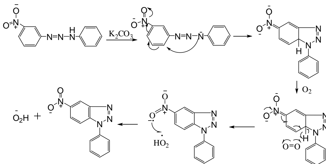
Scheme 2. Plausible mechanism
