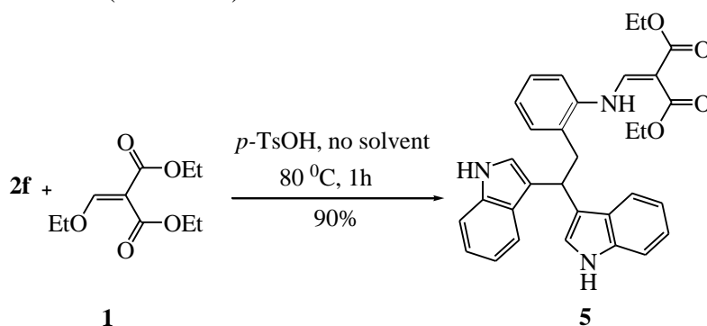
Scheme 4. Reaction of 1 H -indole with DEEM
