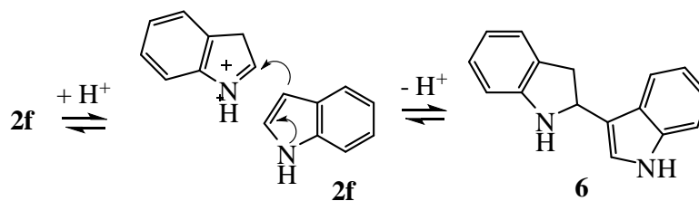
Scheme 5. 1 H -indole/indole dimer equilibrium
