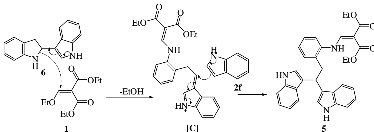
Scheme 6. Plausible mechanism for the formation of 5
