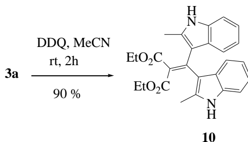
Scheme 8 Oxidation of 3a to 10
