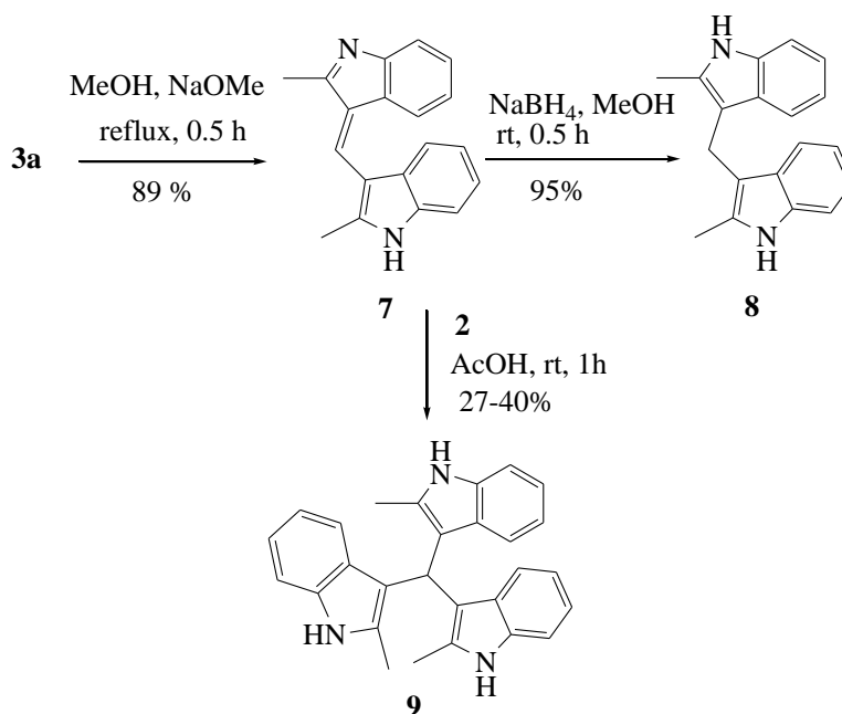
Scheme 7. Synthesis of 8 and 9 from 3a
