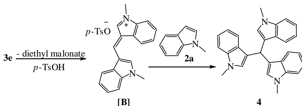
Scheme 3. Formation of tris(1-methylindolyl)methane 4
