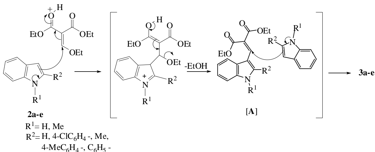
Scheme 2. Plausible mechanism for the formation of 3a-e
