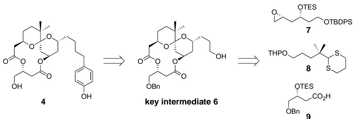
Scheme 1. Retrosynthetic analysis of 4 .
