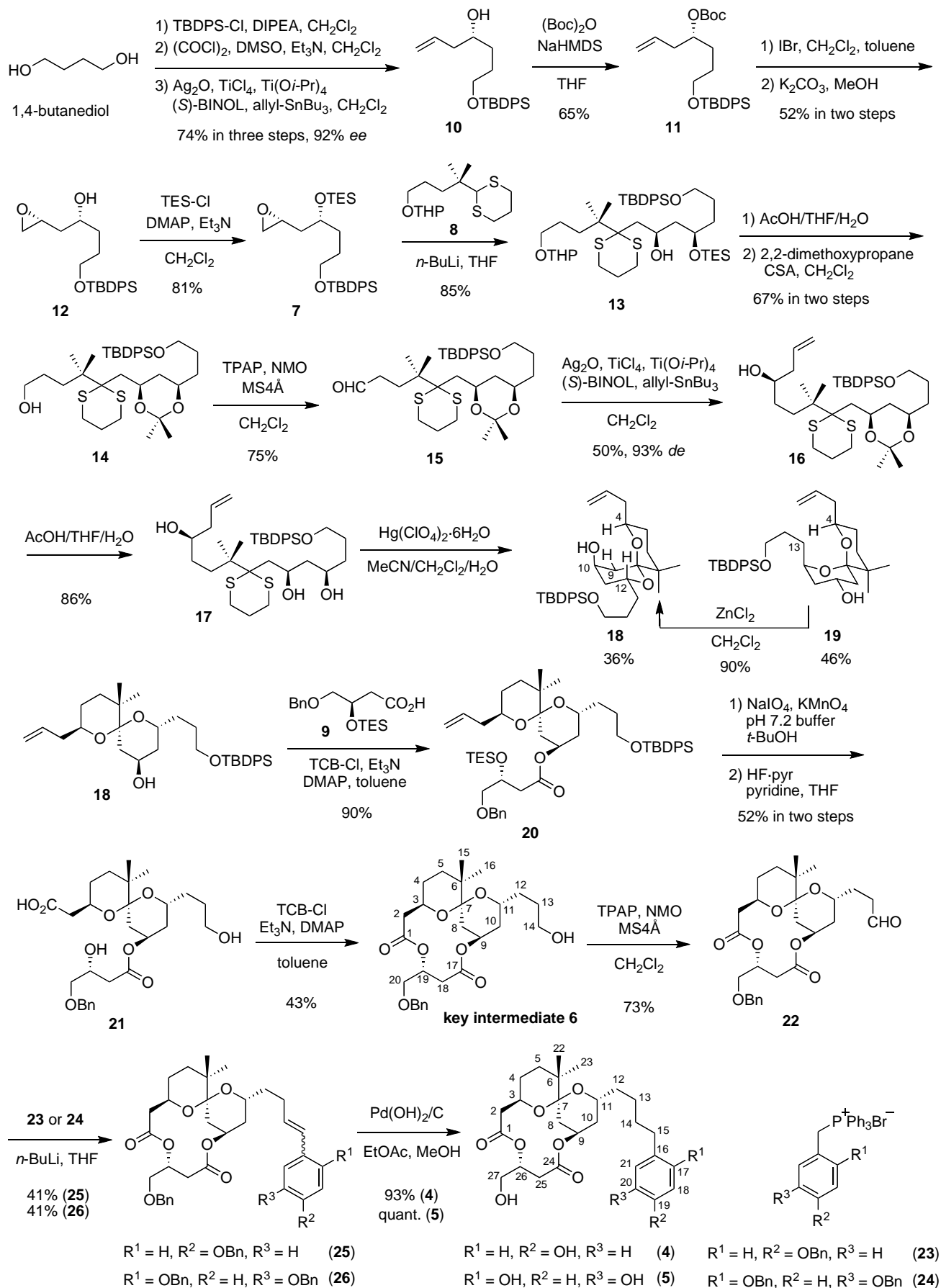
Scheme 2. Synthesis of 4 and 5.
