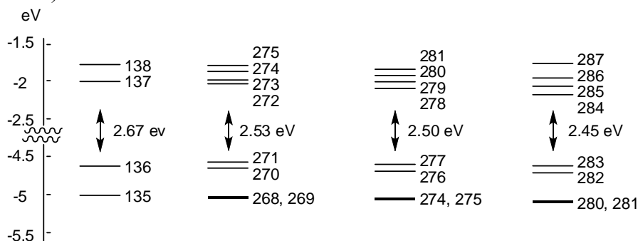
Figure 3. Energy diagrams of 8a (left), 5 (middle left), 6 (middle right), and 7 (right)
