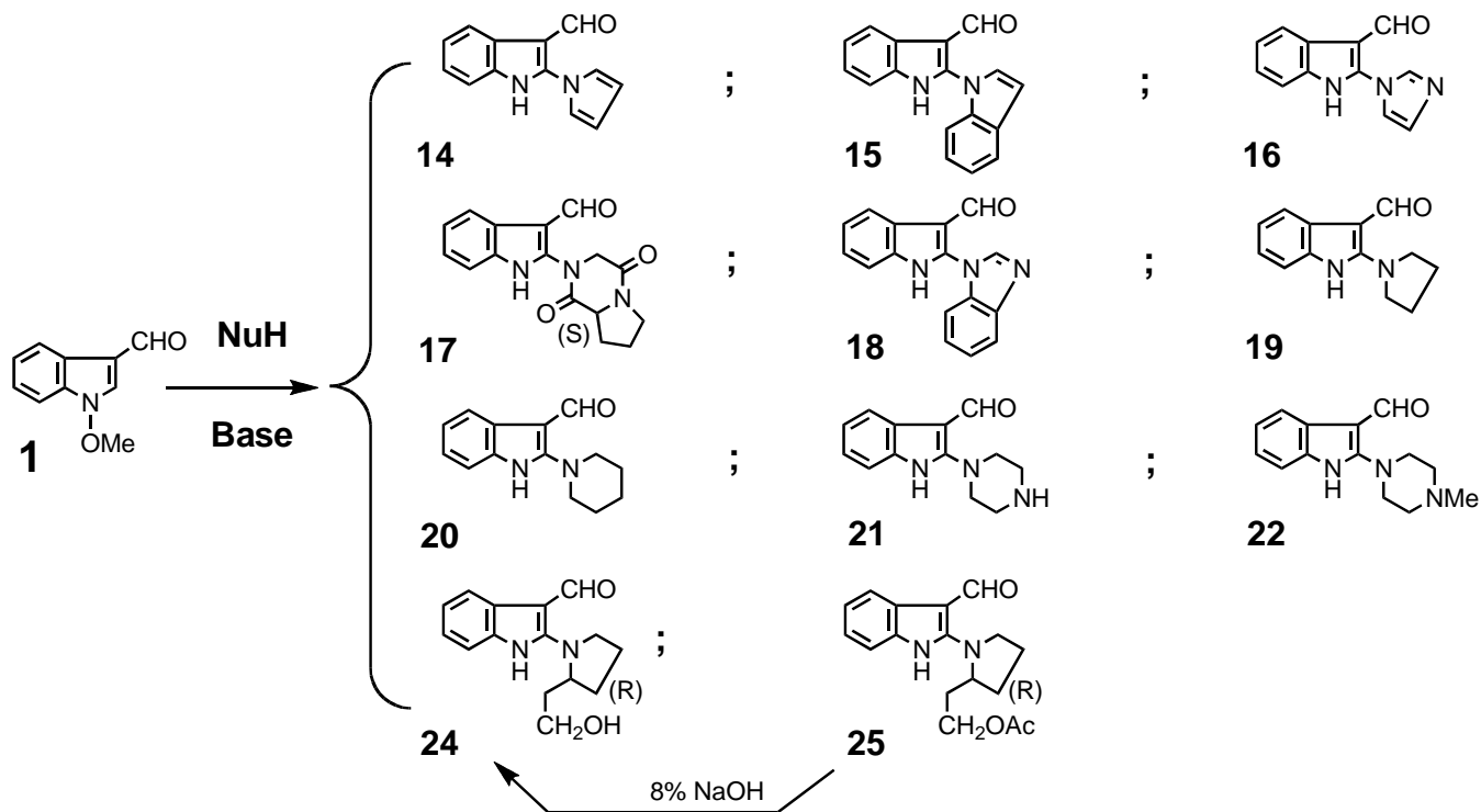
Scheme 3. Reaction of 1 with Nitrogen-Centered Nucleophiles
