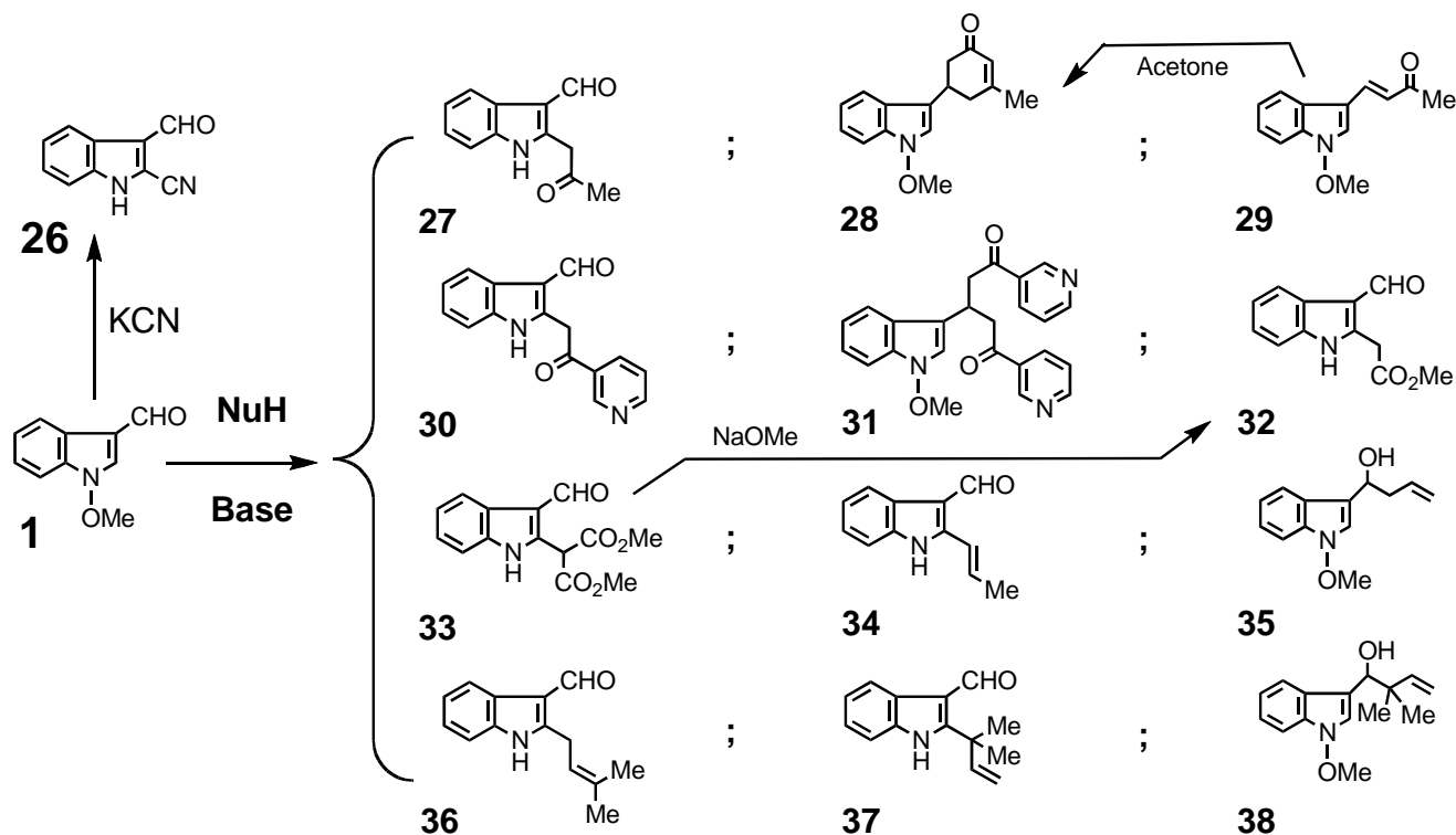
Scheme 5. Reaction of 1 with Carbon-Centered Nucleophiles
