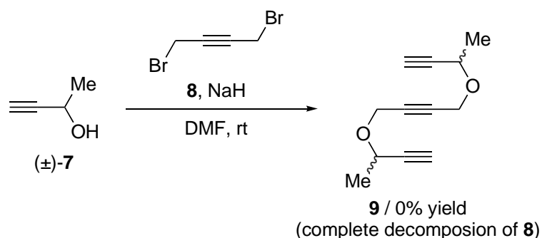
Scheme 4. Reaction of Propargylic Alcohol ( \pm )- 7 with Dibromide 8
