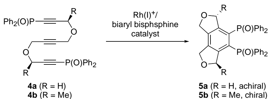
Scheme 2. Rhodium-Catalyzed [2+2+2] Cycloadditions of Triyne Diposphine Oxides 4
