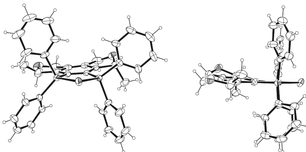
Figure 2. ORTEP diagram of [\text{Rh}(\text{cod})(+)\text{-6b}]\text{SbF}_6 with ellipsoids at 20% probability (left: front view, right: side view): cod and \text{SbF}_6 anion are omitted for clarity.
