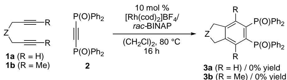
Scheme 1. Rhodium-Catalyzed Reactions of 1,6-Diynes 1 with Bis(diphenylphosphinoyl)acetylene ( 2 )
