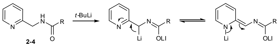
Scheme 3. Resonance forms obtained from 2-4 on reaction with t -BuLi.
