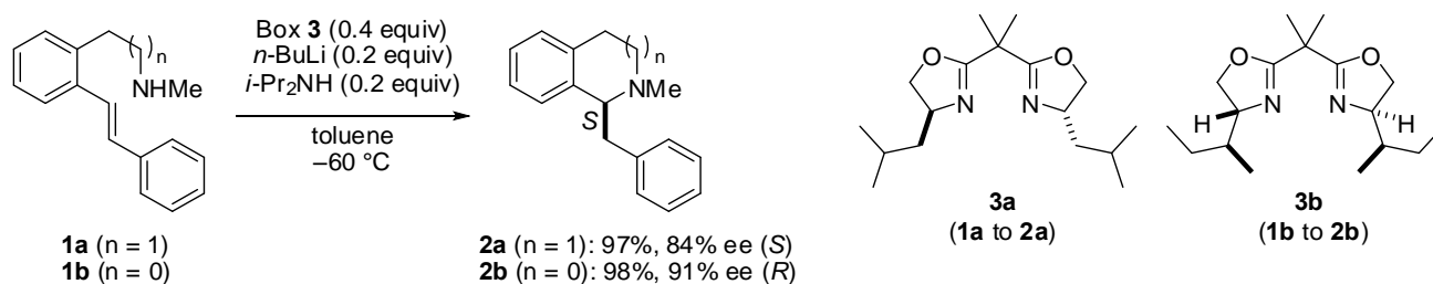
Scheme 1. Chiral box–LDA-catalyzed asymmetric intramolecular hydroamination of aminoalkenes 1 .
