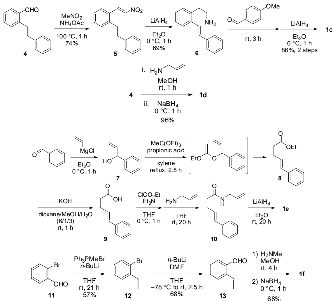
Scheme 2. Synthesis of aminoalkenes 1c–1f .
