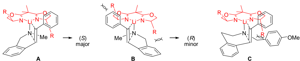
Figure 2. Plausible stereoinduction model for a chiral bisoxazoline–lithium amide-catalyzed asymmetric intramolecular hydroamination.
