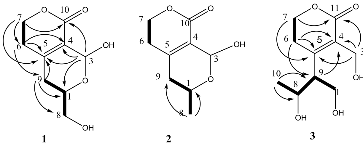
Figure 1. Key HMBC (full-line arrows) and H-H COSY (bold line) correlations of 1 , 2 and 3
