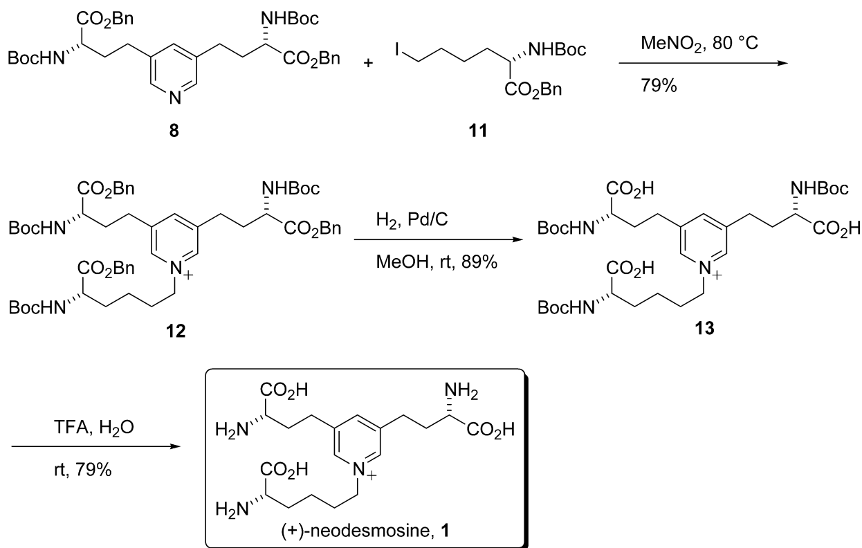
Scheme 2. Total synthesis of neodesmosine 1
