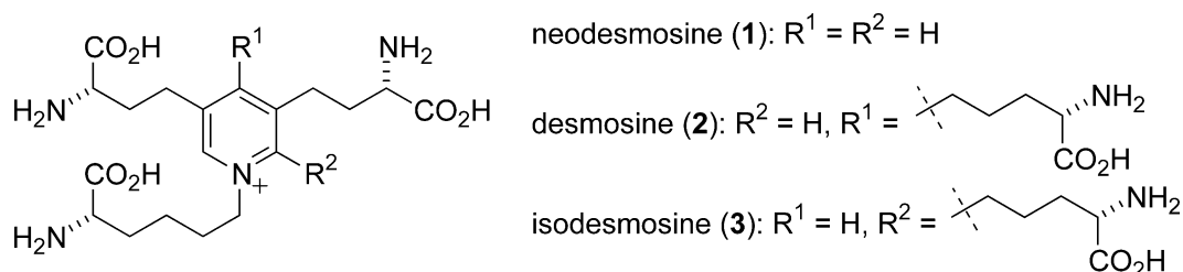
Figure 1. Structures of neodesmosine (1), desmosine (2), and isodesmosine (3)
