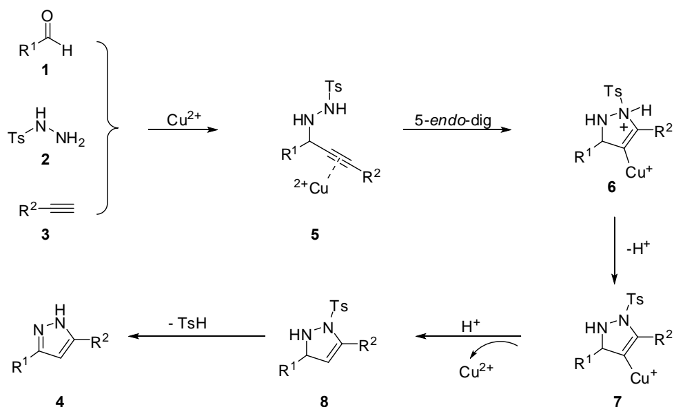
Scheme 1. Proposed mechanism
