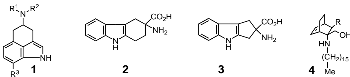
Figure 1 R, R^n = an appropriate substituent
