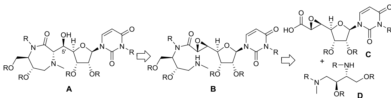
Scheme 1. Synthetic strategy of the diazepanone core of liposidomycins and caprazamycins
