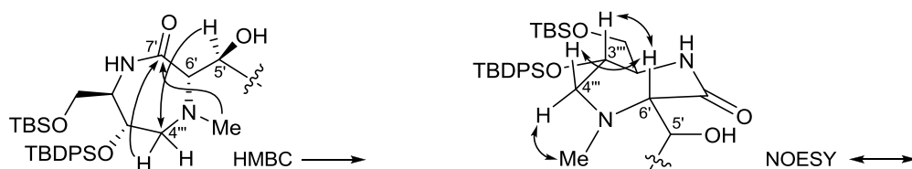
Figure 2. Selected HMBC correlations and NOE correlations of 13
