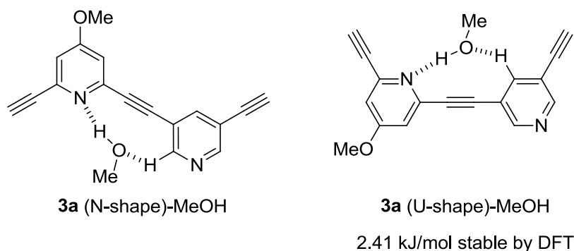
Figure 4. Possible push-pull binding of methanol by pyridine nitrogen and 2- or 4-pyridine C-H represented by model compound 3a with difference of stability predicted by DFT calculation. Conditions: B3LYP/6-31+G(d,p).
