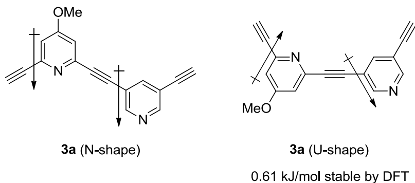
Figure 1. Ethynylpyridine polymers 1 and alternate cooligomers 2 and 3 .
