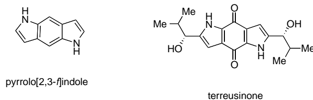
Figure 1. The pyrrolo[2,3-f]indole ring system, and the natural product terreusinone
