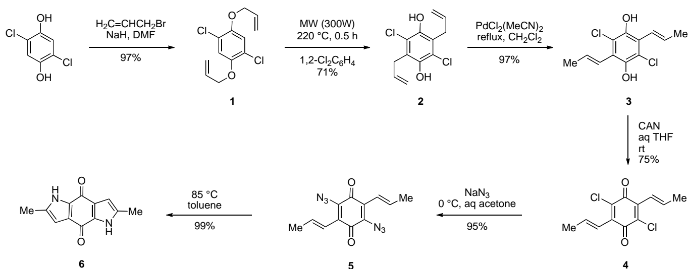
Scheme 1. Double Claisen rearrangement and nitrene cyclization
