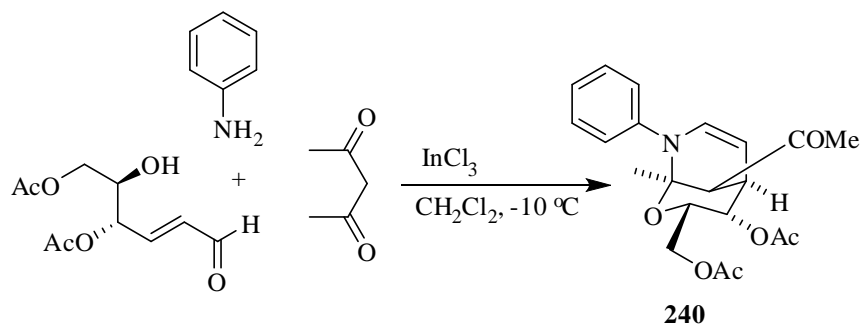
Scheme 195
