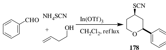
Scheme 143
