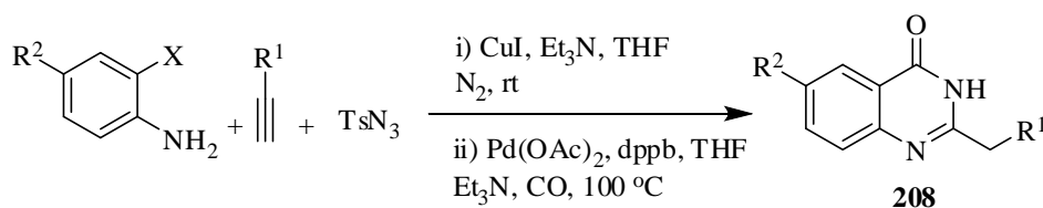
Scheme 165
