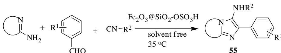
Scheme 45
