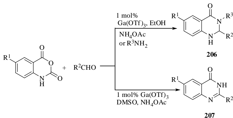
Scheme 164
