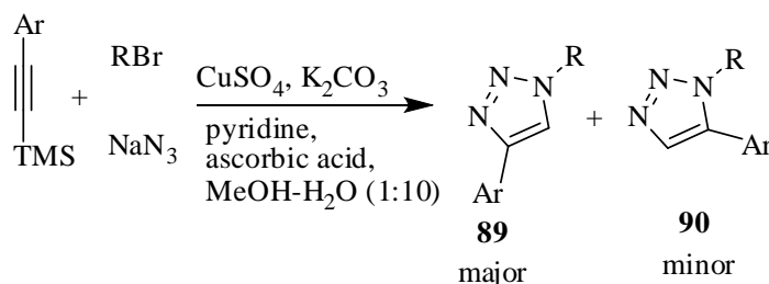
Scheme 73
