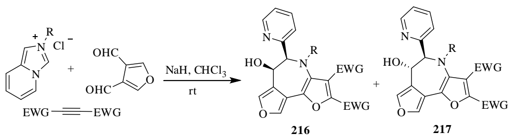
Scheme 173
