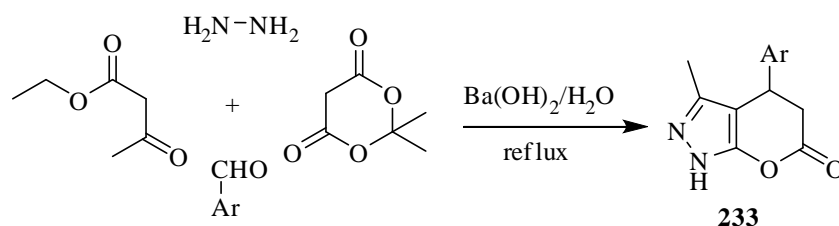
Scheme 188
