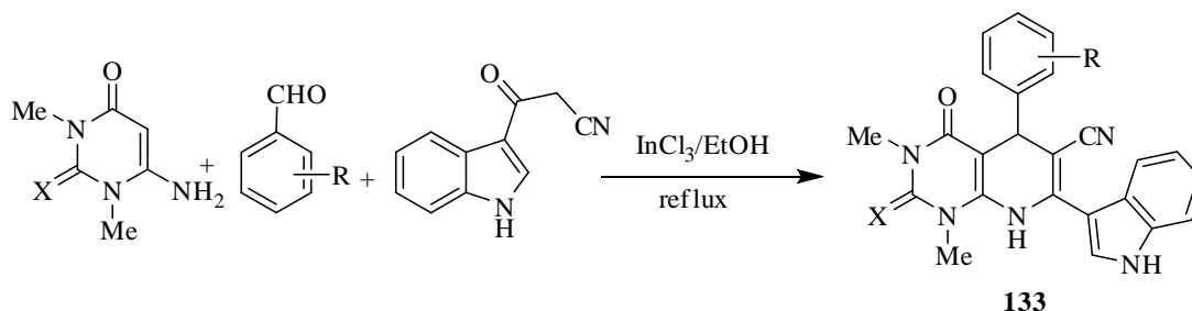
Scheme 107
