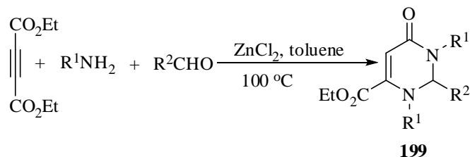
Scheme 159
