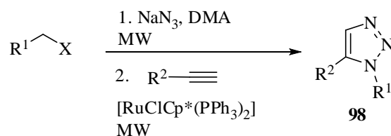
Scheme 79
