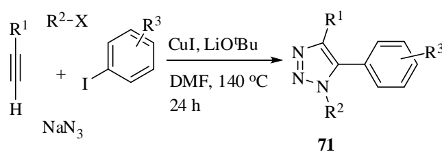
Scheme 59
