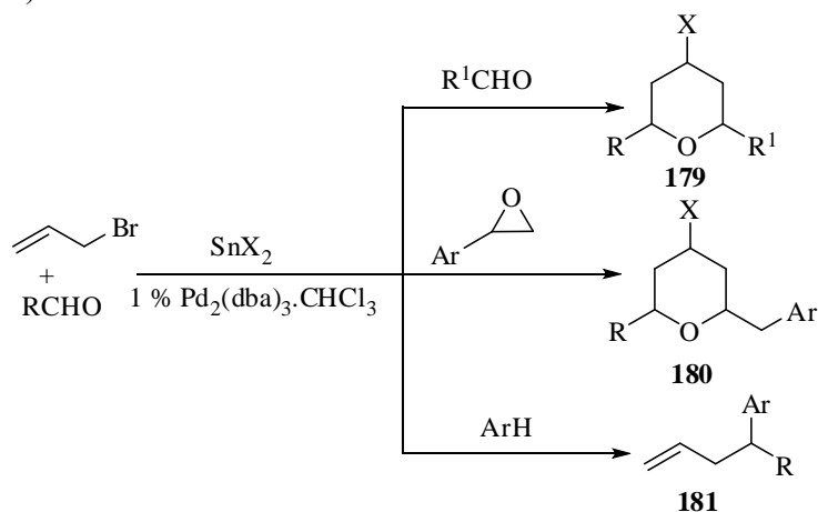
Scheme 144
