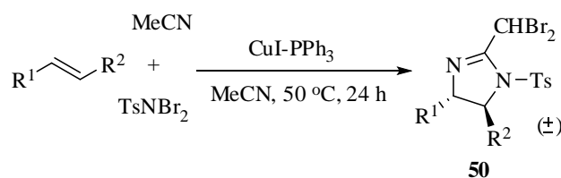
Scheme 41
