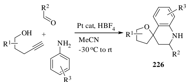
Scheme 181
