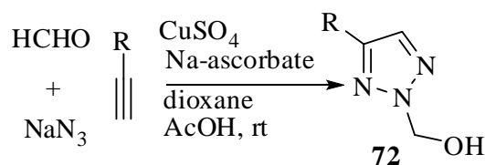
Scheme 60
