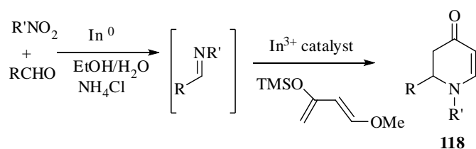
Scheme 98
