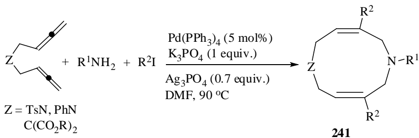
Scheme 196
