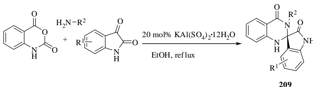
Scheme 166
