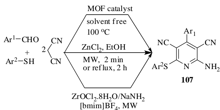
Scheme 88
