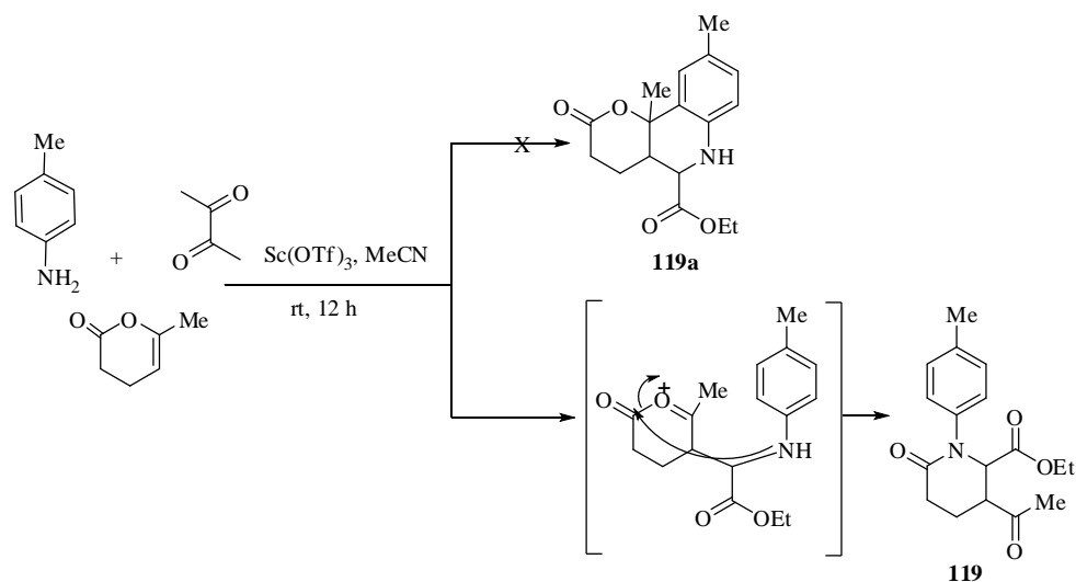
Scheme 99
