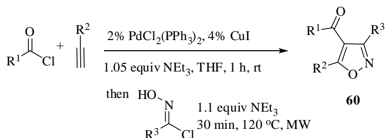
Scheme 50
