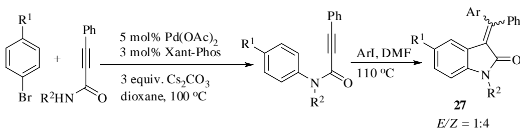
Scheme 21
