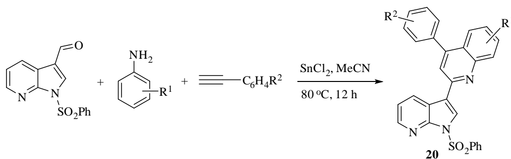
Scheme 15
