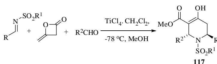
Scheme 97
