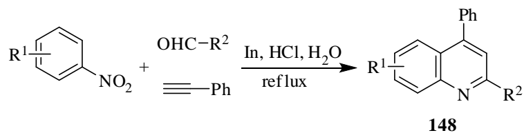
Scheme 119
