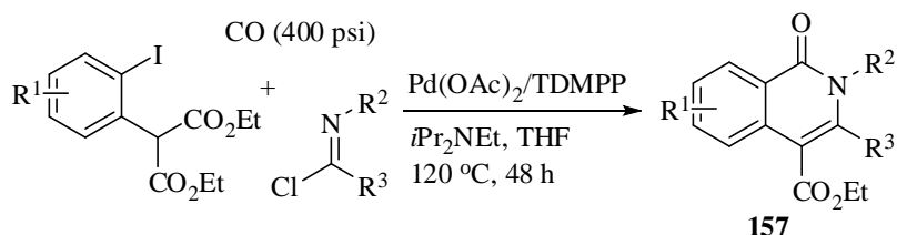
Scheme 127
