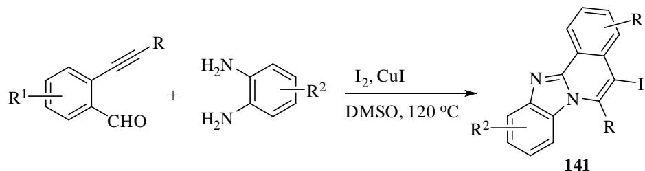
Scheme 114
