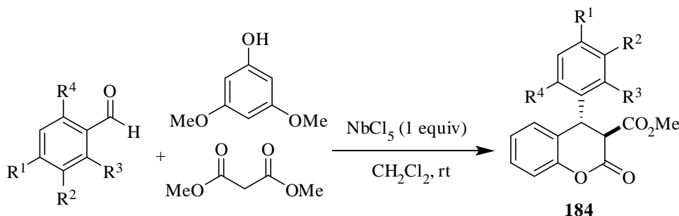
Scheme 147
