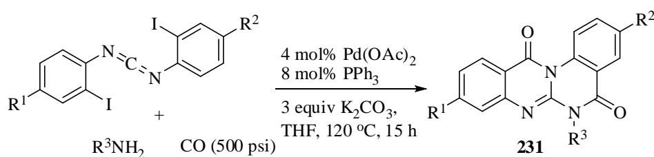
Scheme 186
