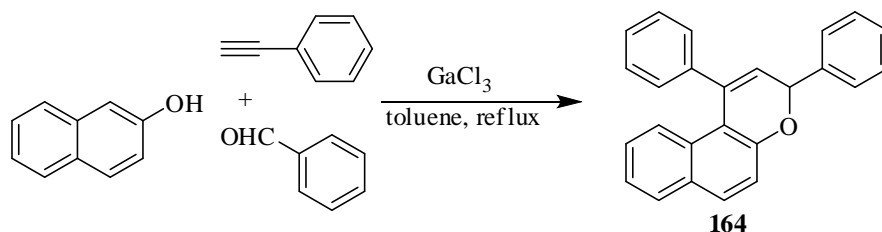
Scheme 132
