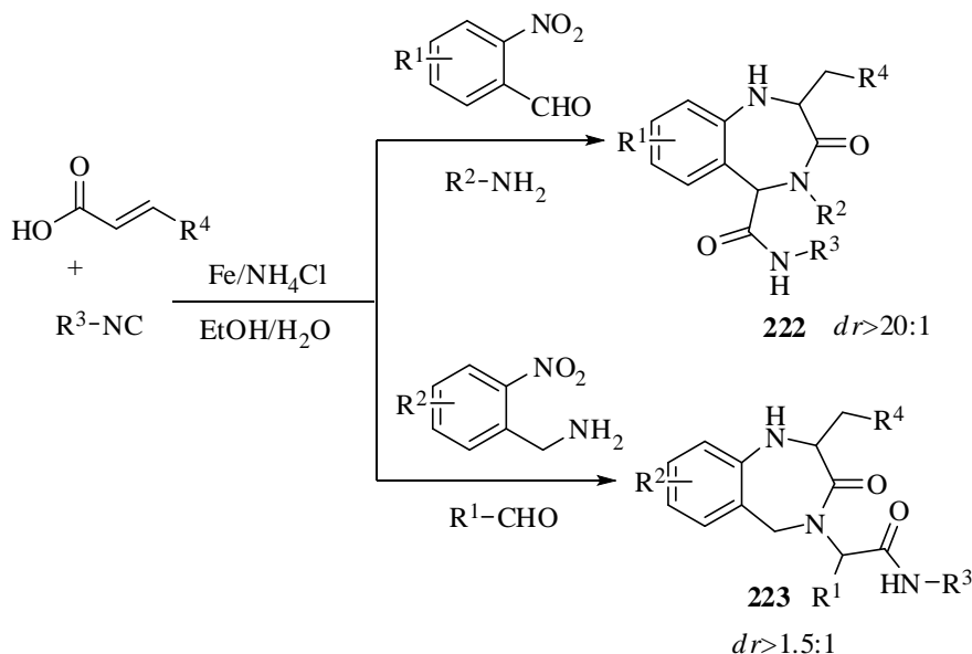
Scheme 178
