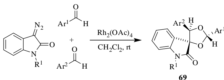
Scheme 57
