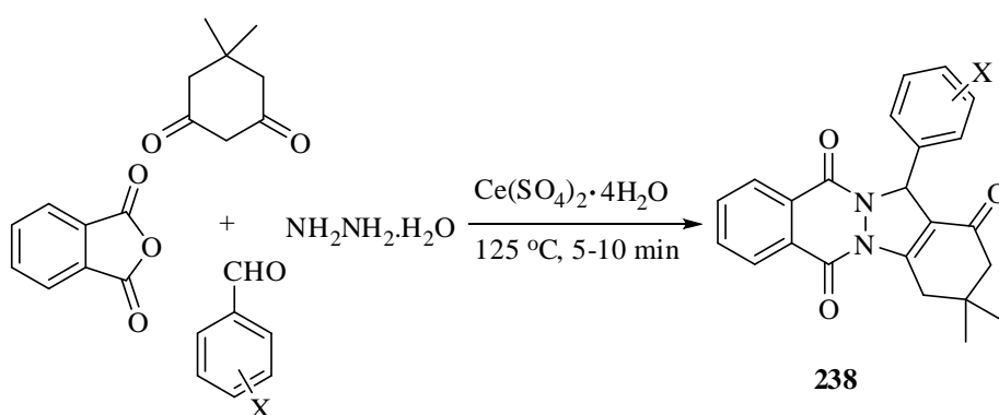
Scheme 193
