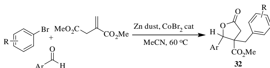
Scheme 24
