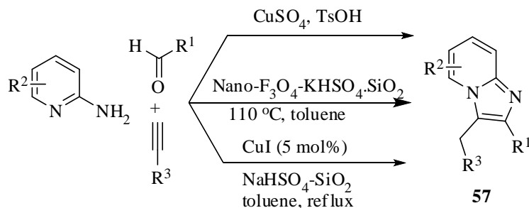
Scheme 47
