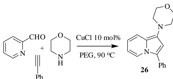
Scheme 20
