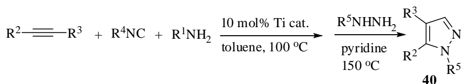
Scheme 32
