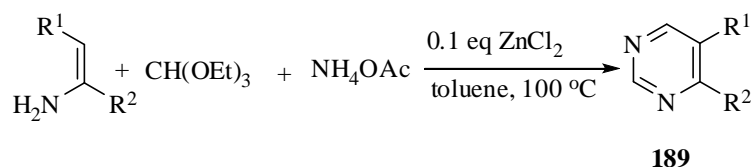
Scheme 151
