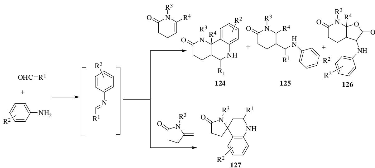
Scheme 102
