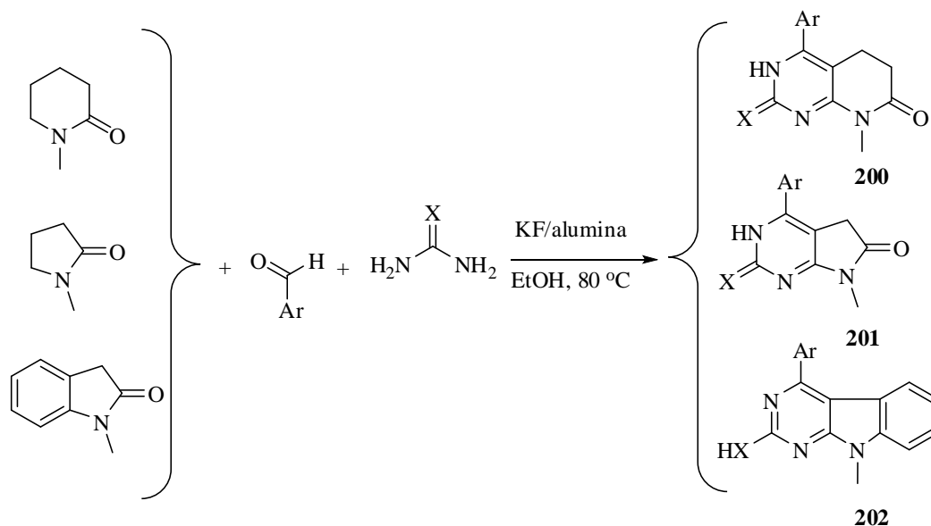
Scheme 160
