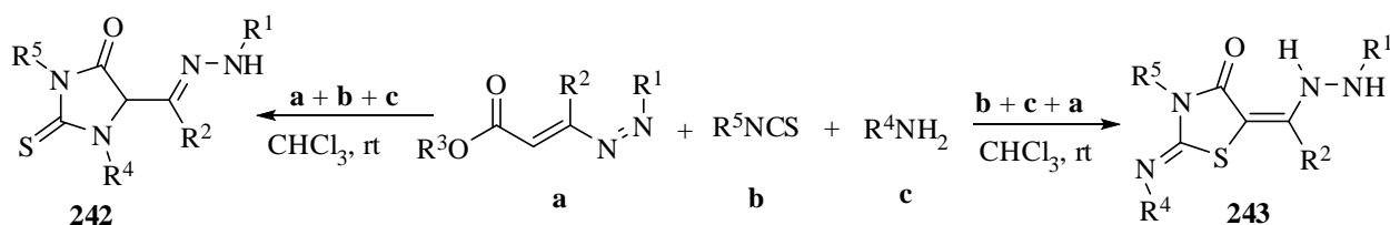
Scheme 197
