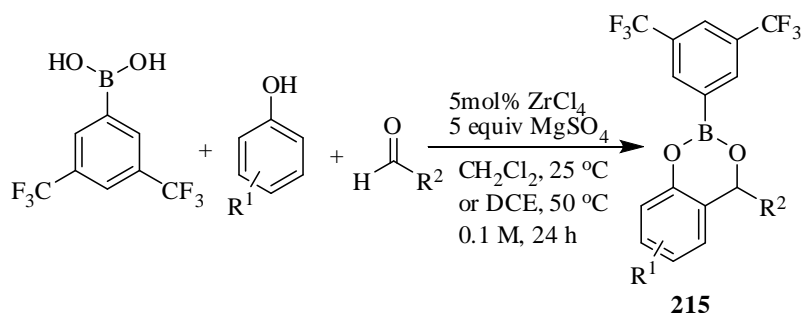
Scheme 172
