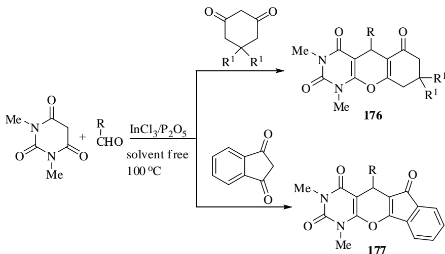
Scheme 142
