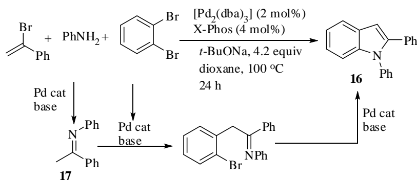
Scheme 12
