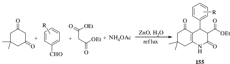
Scheme 125
