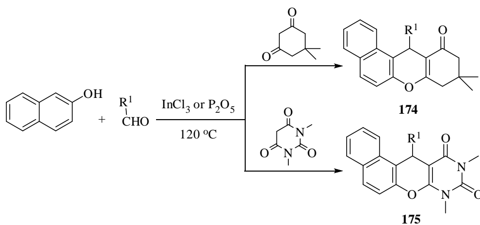
Scheme 141
