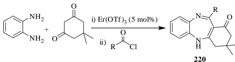
Scheme 176
