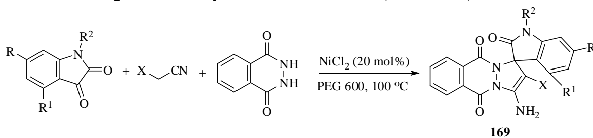
Scheme 137
