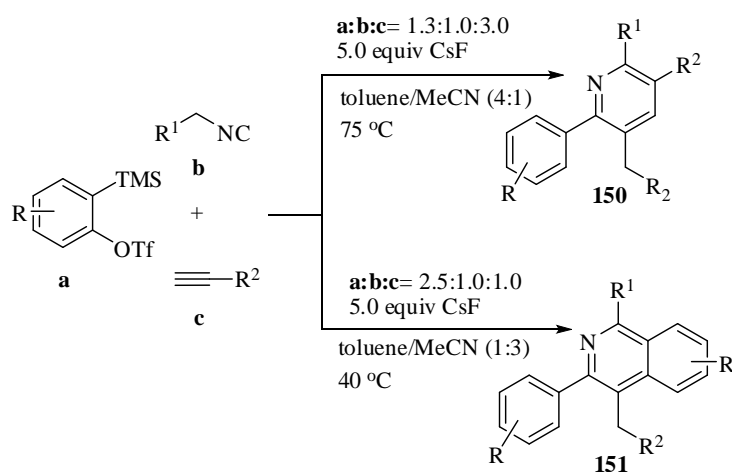
Scheme 121
