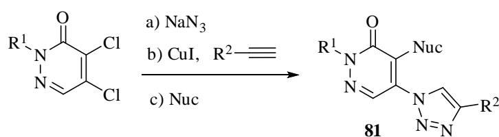
Scheme 68
