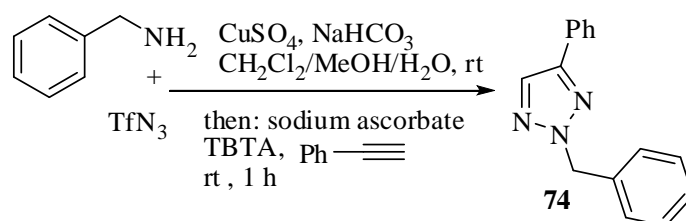
Scheme 62
