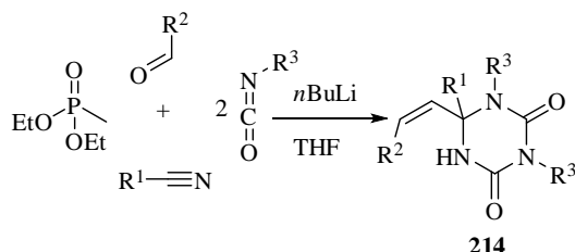
Scheme 171
