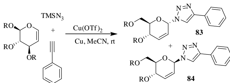
Scheme 70
